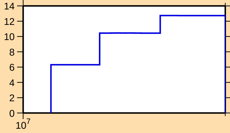
\Delta\sigma/\sigma vs. E for ^{120}\text{Xe}(n,\text{tot.})
