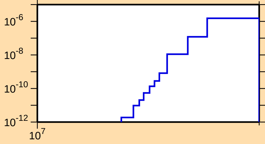
\sigma vs. E for ^{120}\text{Xe}(\text{mt 45})
