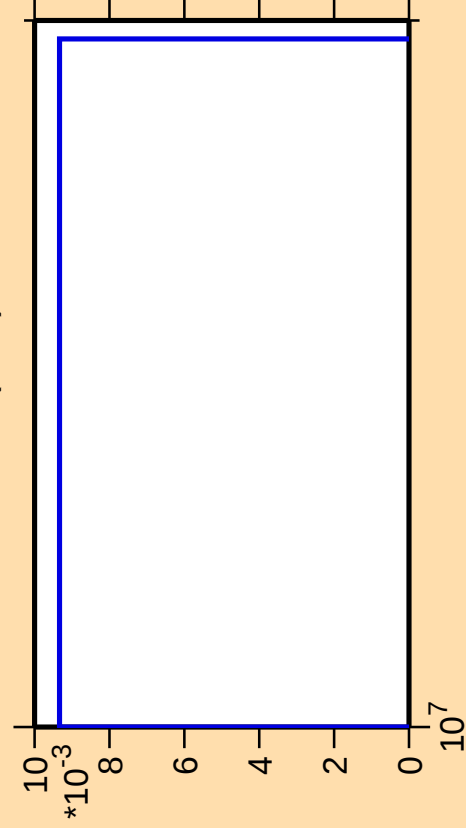
\Delta\sigma/\sigma vs. E for ^{120}\text{Xe}(n,nt)
