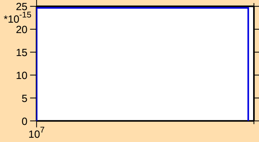
\sigma vs. E for ^{120}\text{Xe}(\text{mt 34})
