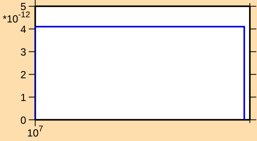
\sigma vs. E for ^{120}\text{Xe}(n,\text{pt})
