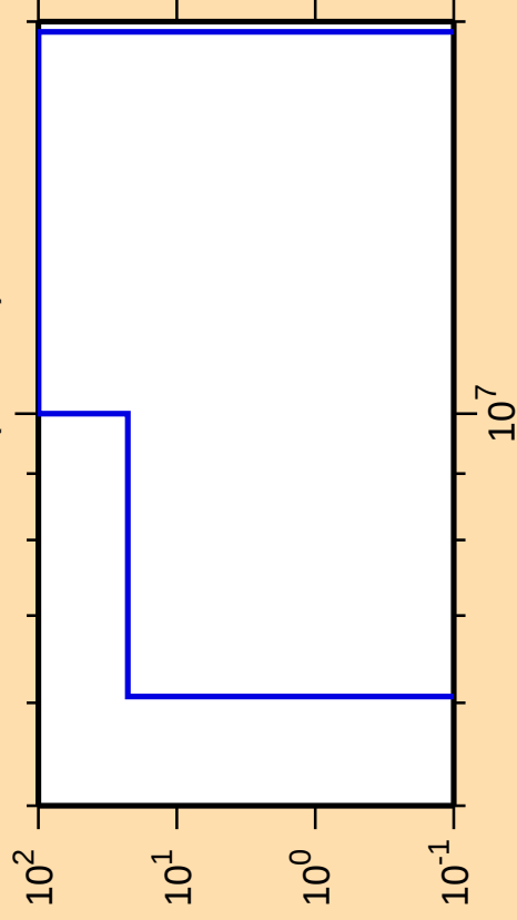
\Delta\sigma/\sigma vs. E for ^{120}\text{Xe}(n,\text{He}3)
