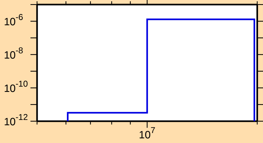
\sigma vs. E for ^{120}\text{Xe}(n,\text{He}3)
