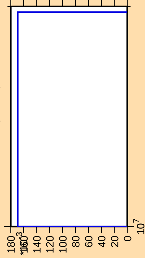
\Delta\sigma/\sigma vs. E for ^{120}\text{Xe}(\text{mt 34})
