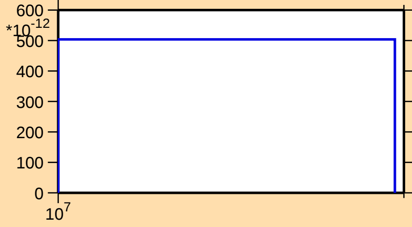
\sigma vs. E for ^{120}\text{Xe}(n,2np)
