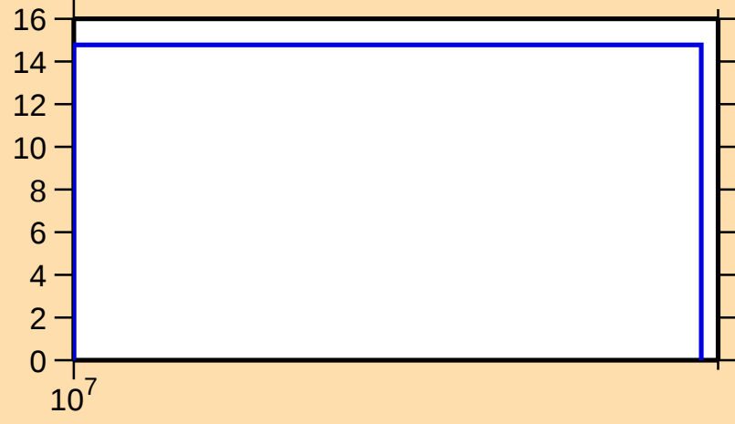
\Delta\sigma/\sigma vs. E for ^{120}\text{Xe}(n,\text{nonel.})
