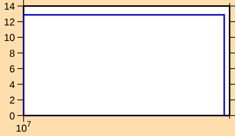
\Delta\sigma/\sigma vs. E for ^{120}\text{Xe}(n,\text{el.})
