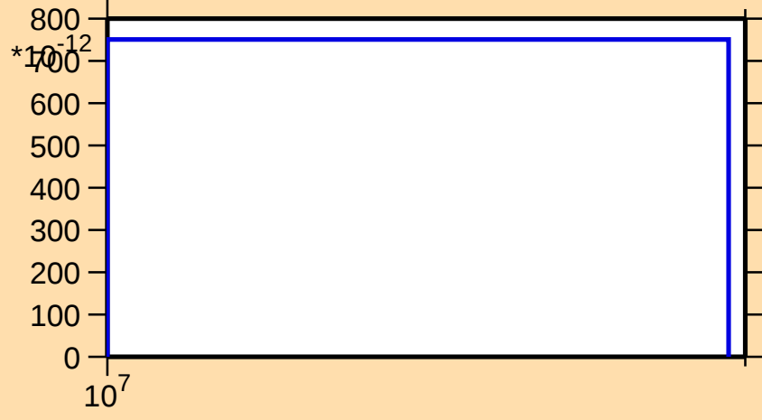
\sigma vs. E for ^{120}\text{Xe}(n,2n\alpha)
