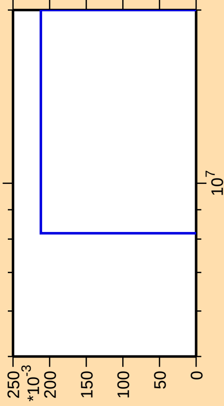
\Delta\sigma/\sigma vs. E for ^{120}\text{Xe}(\text{mt } 34)
