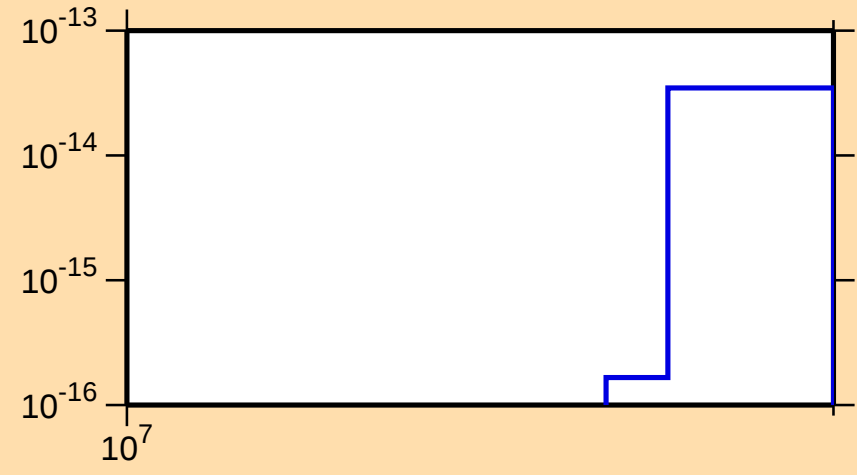
\sigma vs. E for ^{122}\text{Xe}(\text{mt } 34)
