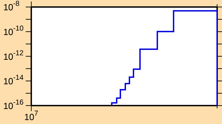
\sigma vs. E for ^{122}\text{Xe}(\text{mt } 45)
