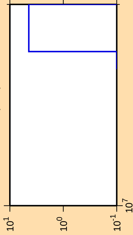
\Delta\sigma/\sigma vs. E for ^{122}\text{Xe}(n,nt)
