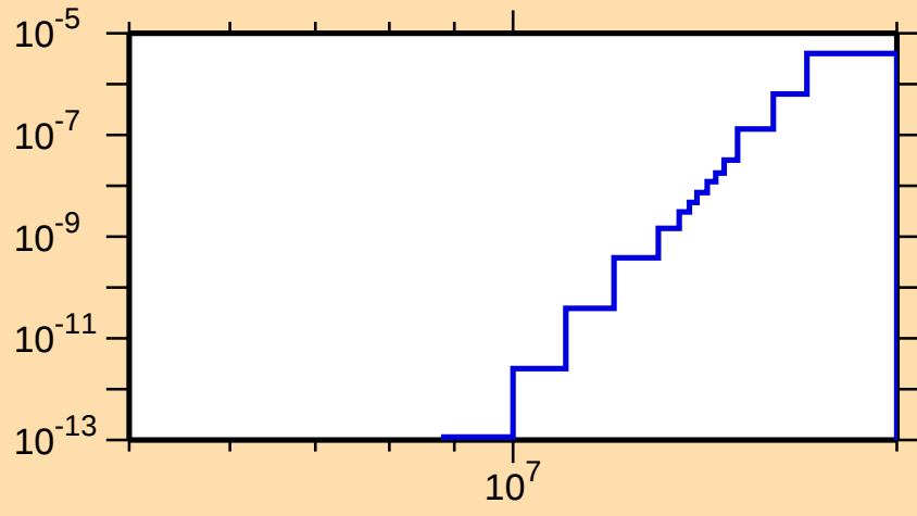
\sigma vs. E for ^{122}\text{Xe}(n,\text{He3})
