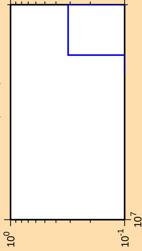
\Delta\sigma/\sigma vs. E for ^{122}\text{Xe}(\text{mt } 34)
