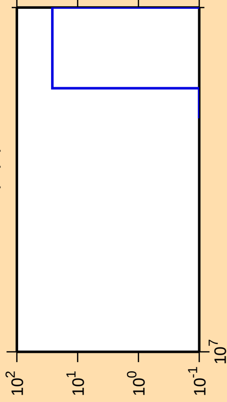
\Delta\sigma/\sigma vs. E for ^{122}\text{Xe}(n,\text{pt})
