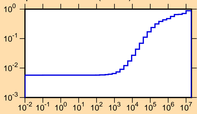
\mu vs. E for ^{122}\text{Xe}(\text{mt251})
