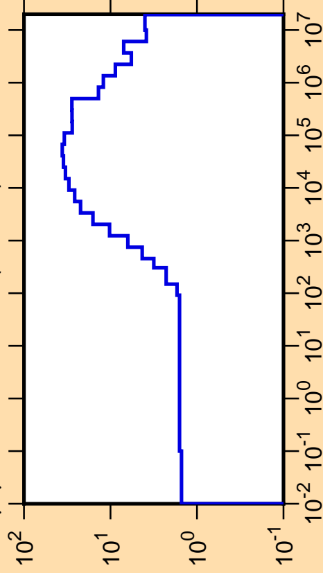
\Delta\mu/\mu vs. E for ^{122}\text{Xe}(\text{mt251})
