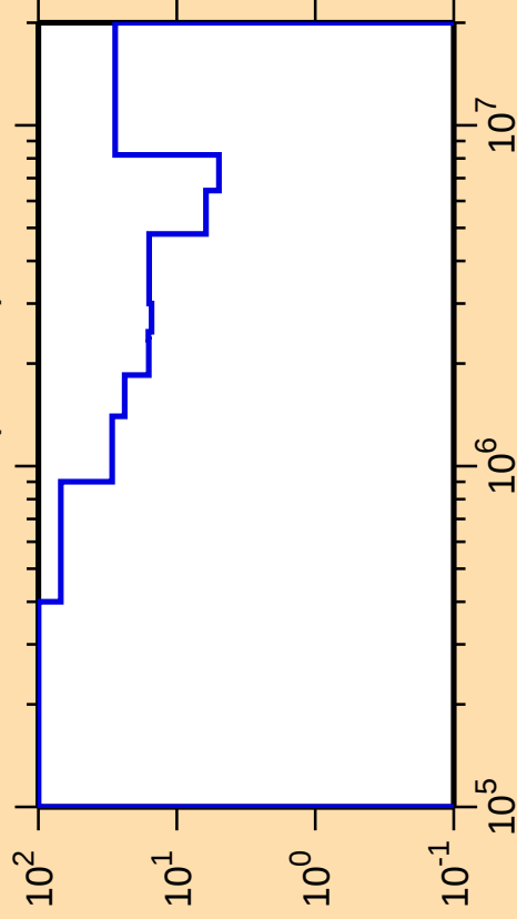
\Delta\sigma/\sigma vs. E for ^{122}\text{Xe}(n,\text{inel.})
