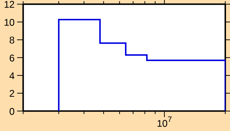
\Delta\sigma/\sigma vs. E for ^{122}\text{Xe}(n,n\text{nonel.})
