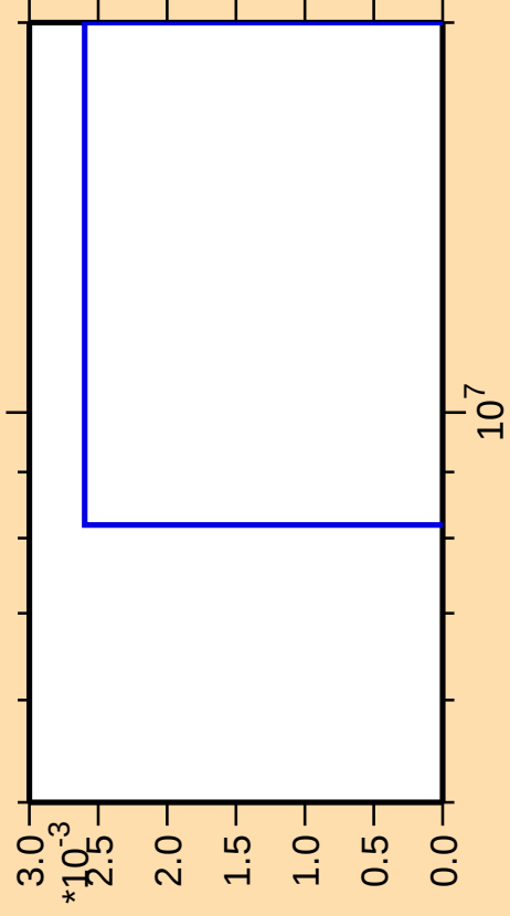
\Delta\sigma/\sigma vs. E for ^{122}\text{Xe}(\text{mt } 34)
