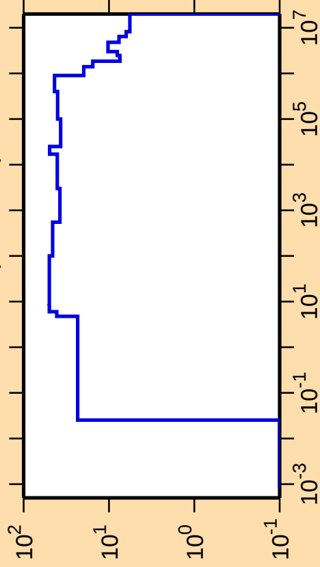
\Delta\sigma/\sigma vs. E for ^{122}\text{Xe}(n,\text{nonel.})
