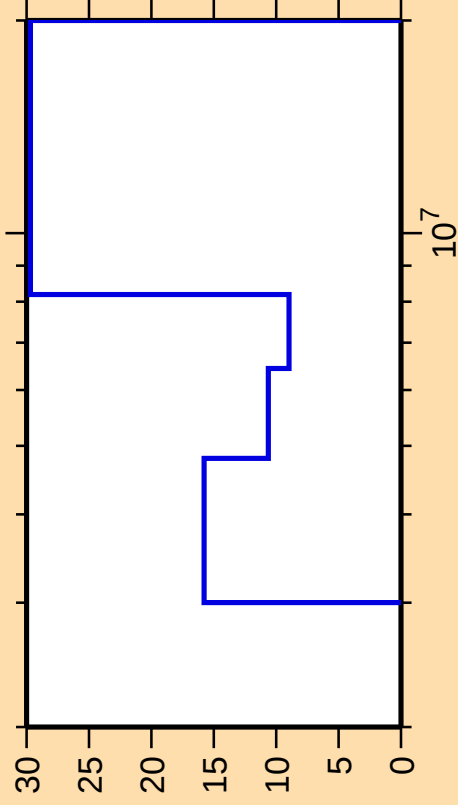
\Delta\sigma/\sigma vs. E for ^{122}\text{Xe}(n,\text{ncont.})
