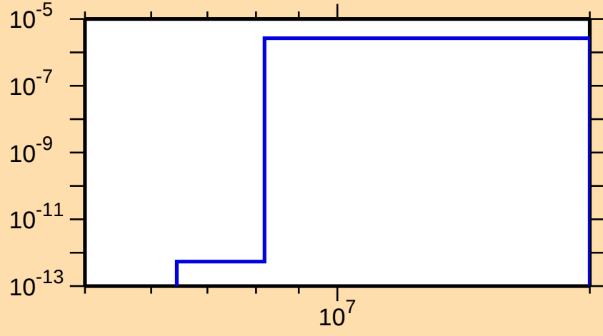
\sigma vs. E for ^{122}\text{Xe}(n,p\alpha)
