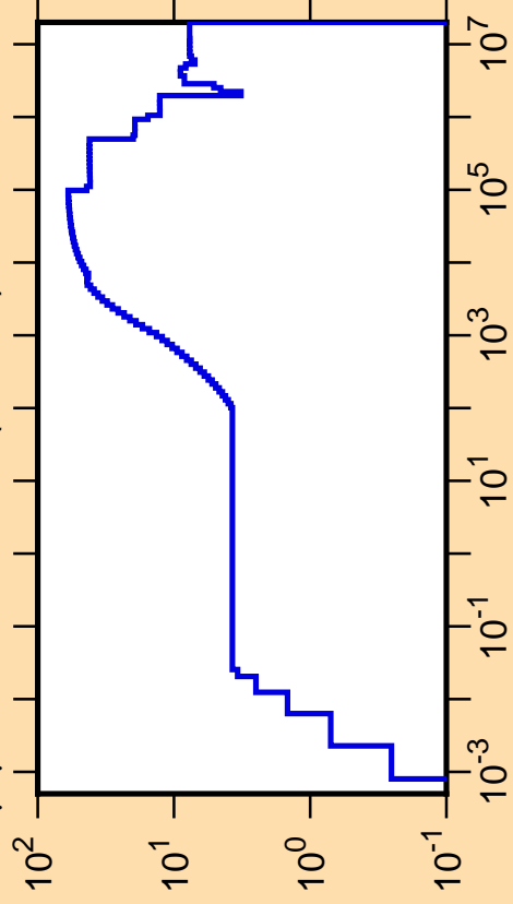
\Delta\mu/\mu vs. E for ^{125}\text{Xe}(\text{mt251})
