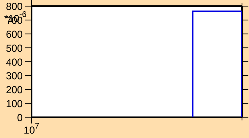
\sigma vs. E for ^{125}\text{Xe}(n,3n)
