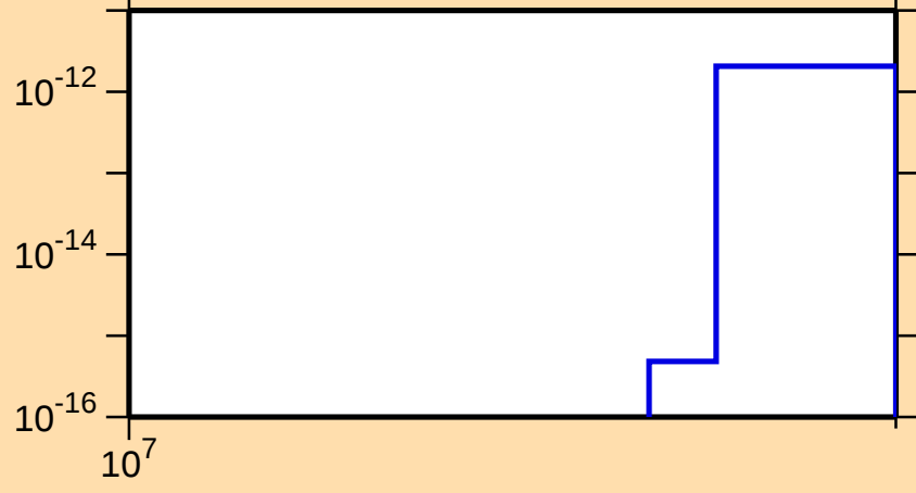
\sigma vs. E for ^{125}\text{Xe}(\text{mt 34})
