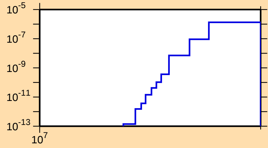
\sigma vs. E for ^{125}\text{Xe}(n,2n\alpha)
