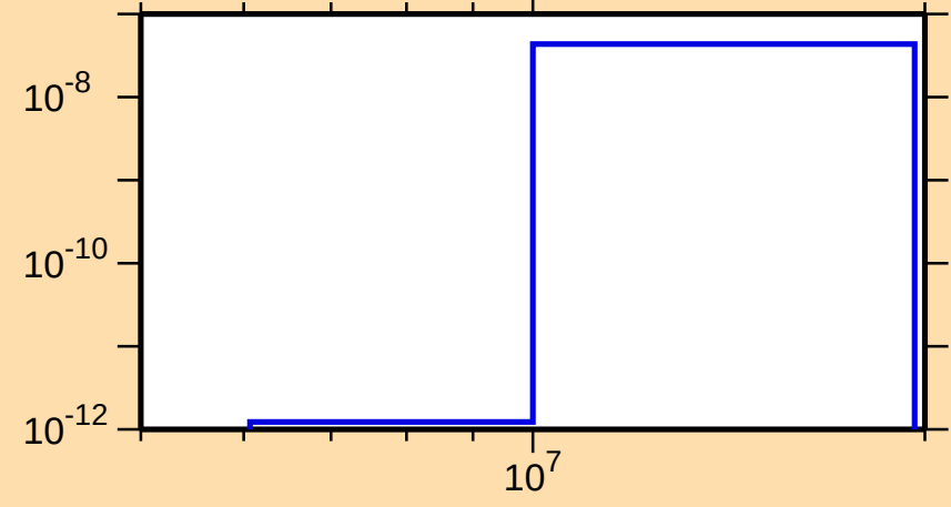
\sigma vs. E for ^{125}\text{Xe}(n,p\alpha)
