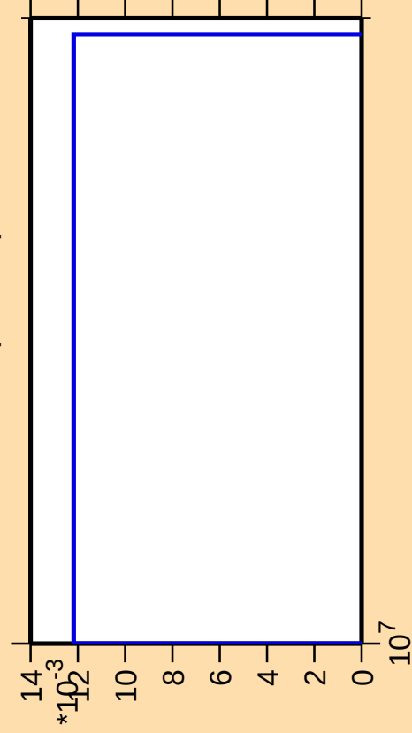
\Delta\sigma/\sigma vs. E for ^{125}\text{Xe}(\text{mt117})
