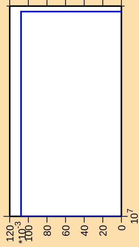
\Delta\sigma/\sigma vs. E for ^{125}\text{Xe}(\text{mt } 34)
