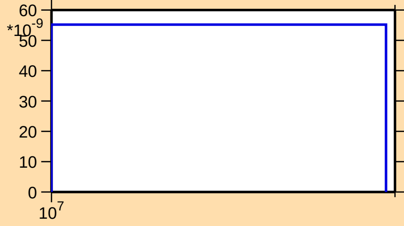
\sigma vs. E for ^{125}\text{Xe}(n,\text{nd})
