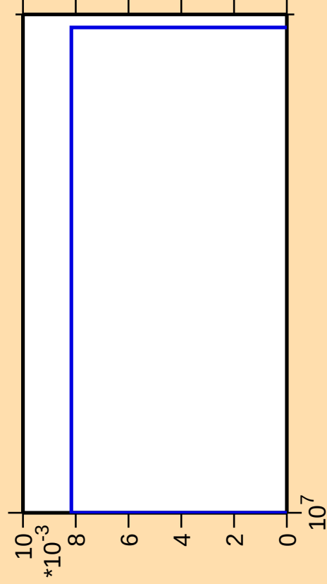
\Delta\sigma/\sigma vs. E for ^{125}\text{Xe}(\text{mt } 45)
