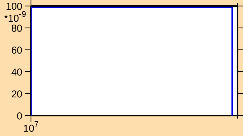
\sigma vs. E for ^{125}\text{Xe}(n,2np)
