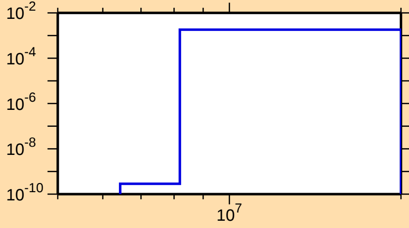
\sigma vs. E for ^{125}\text{Xe}(n,d)
