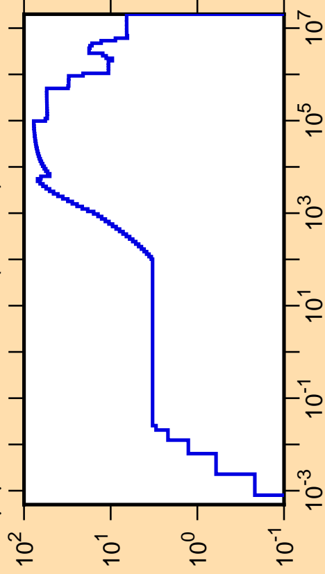
\Delta\mu/\mu vs. E for ^{126}\text{Xe}(\text{mt251})
