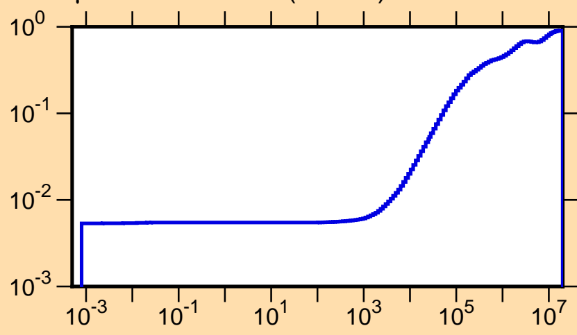
\mu vs. E for ^{126}\text{Xe}(\text{mt251})
