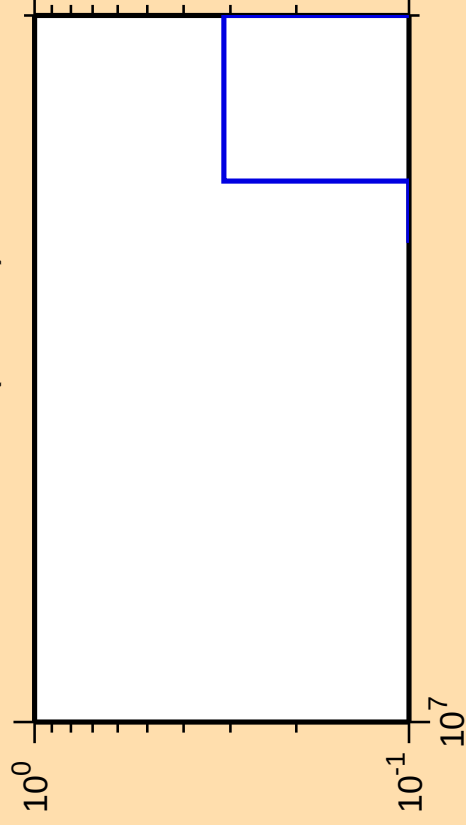
\Delta\sigma/\sigma vs. E for ^{126}\text{Xe}(\text{mt117})
