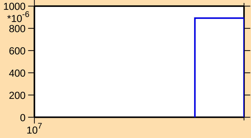
\sigma vs. E for ^{126}\text{Xe}(n,3n)
