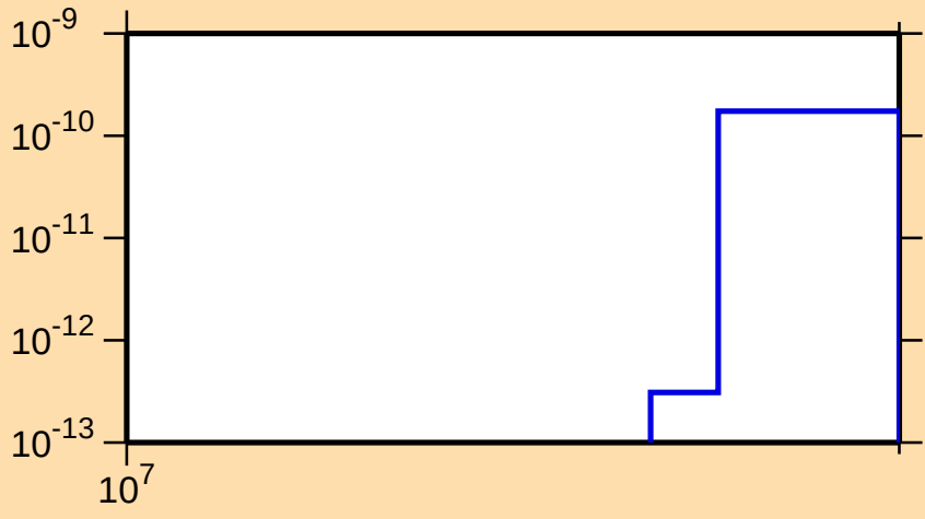
\sigma vs. E for ^{126}\text{Xe}(n,\text{pd})
