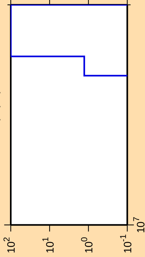
\Delta\sigma/\sigma vs. E for ^{126}\text{Xe}(n,\text{pd})
