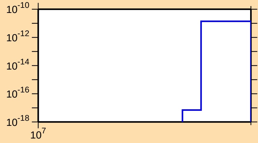
\sigma vs. E for ^{126}\text{Xe}(n,nt)
