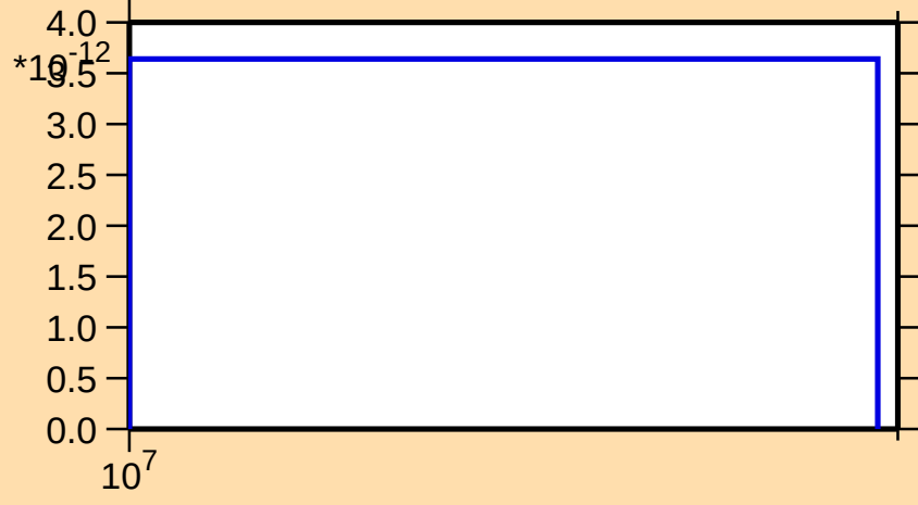
\sigma vs. E for ^{126}\text{Xe}(n,2n\alpha)
