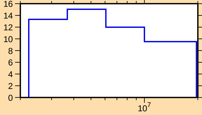
\Delta\sigma/\sigma vs. E for ^{126}\text{Xe}(n,n\text{nonel.})
