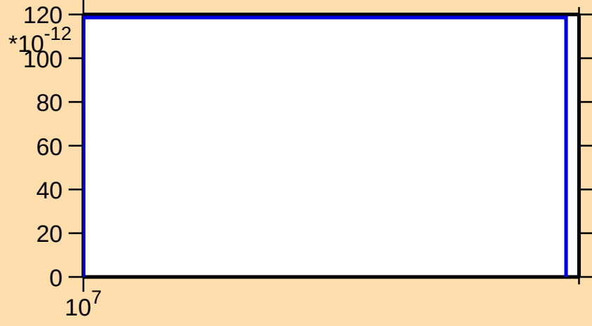
\sigma vs. E for ^{126}\text{Xe}(n,\text{nd})
