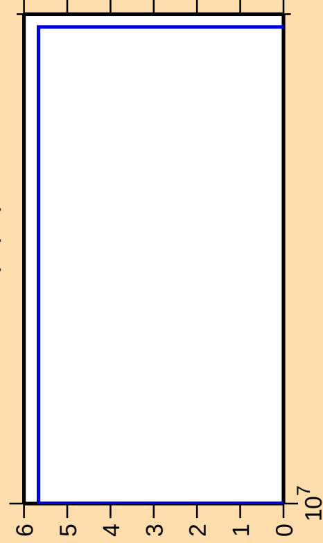
\Delta\sigma/\sigma vs. E for ^{126}\text{Xe}(n,\text{pd})
