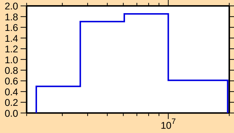
\sigma vs. E for ^{126}\text{Xe}(n,n\text{cont.})
