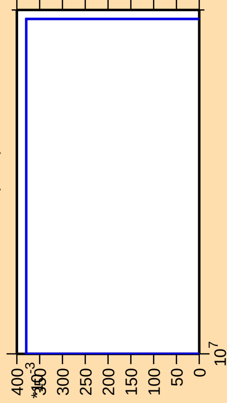
\Delta\sigma/\sigma vs. E for ^{126}\text{Xe}(n,nt)
