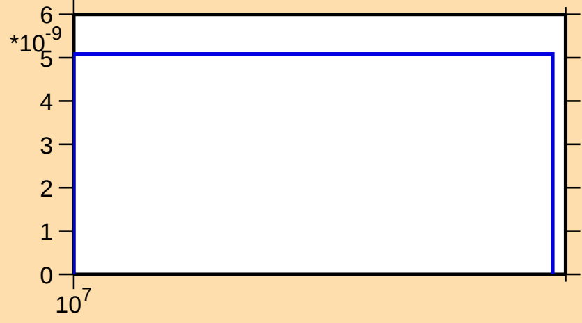
\sigma vs. E for ^{126}\text{Xe}(n,\text{He3})
