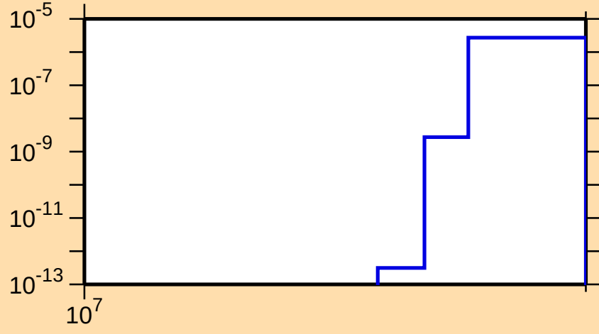
\sigma vs. E for ^{127}\text{Xe}(n,2np)
