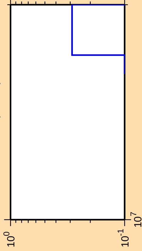
\Delta\sigma/\sigma vs. E for ^{127}\text{Xe}(\text{mt 34})
