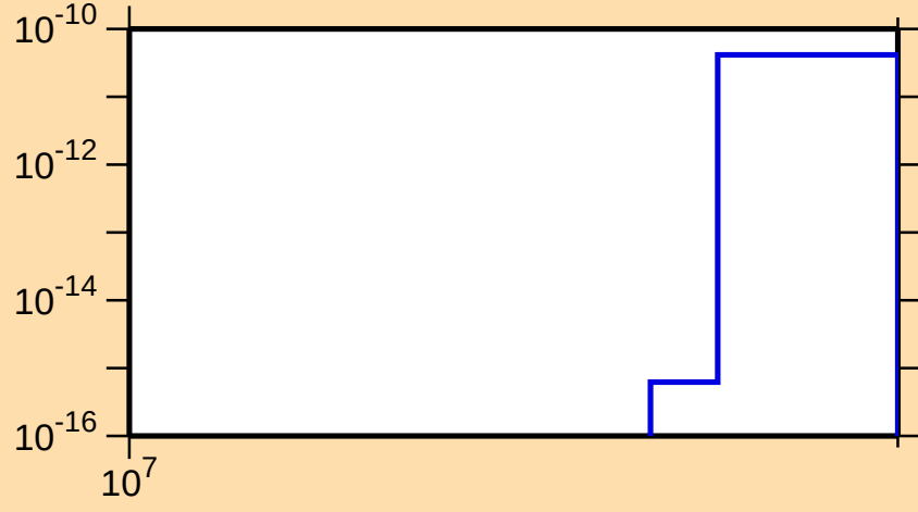
\sigma vs. E for ^{127}\text{Xe}(n,\text{nt})
