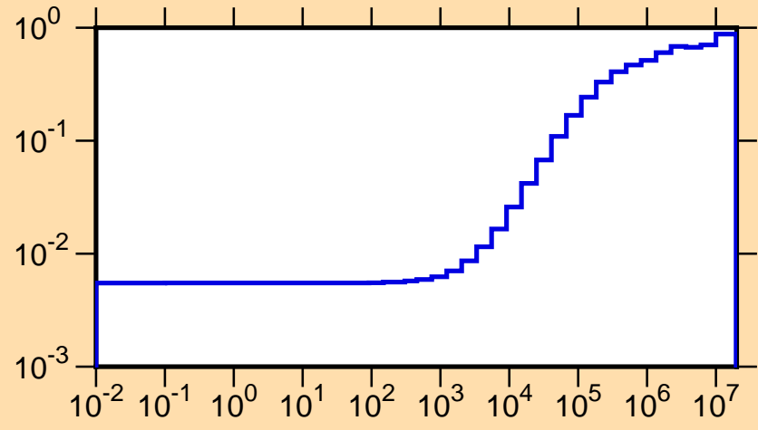
\mu vs. E for ^{127}\text{Xe}(\text{mt251})
