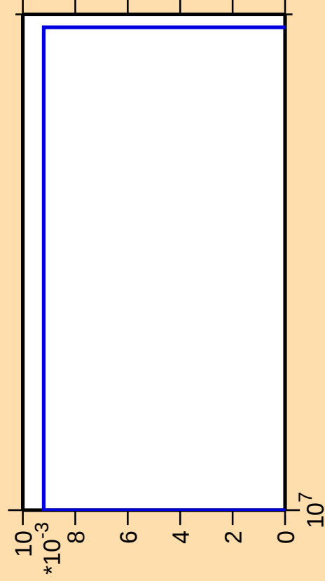
\Delta\sigma/\sigma vs. E for ^{127}\text{Xe}(n,\text{pd})
