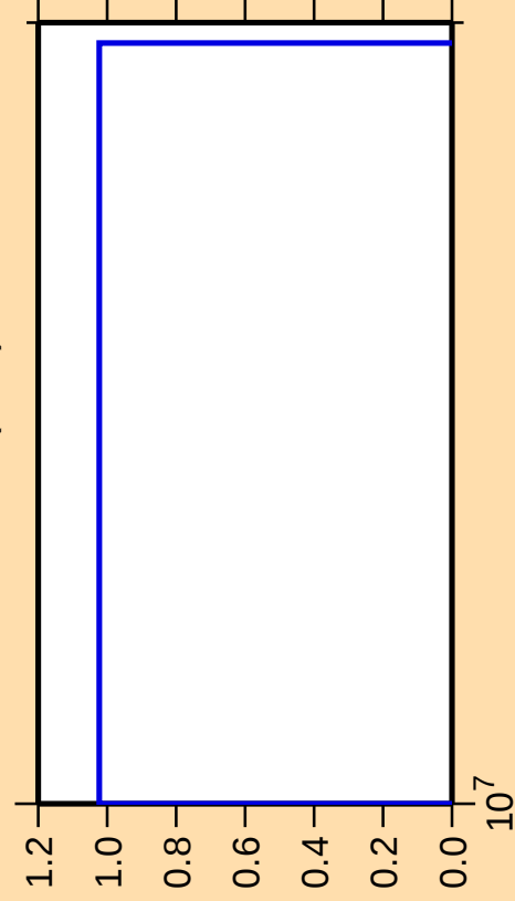
\Delta\sigma/\sigma vs. E for ^{127}\text{Xe}(n,\text{nt})
