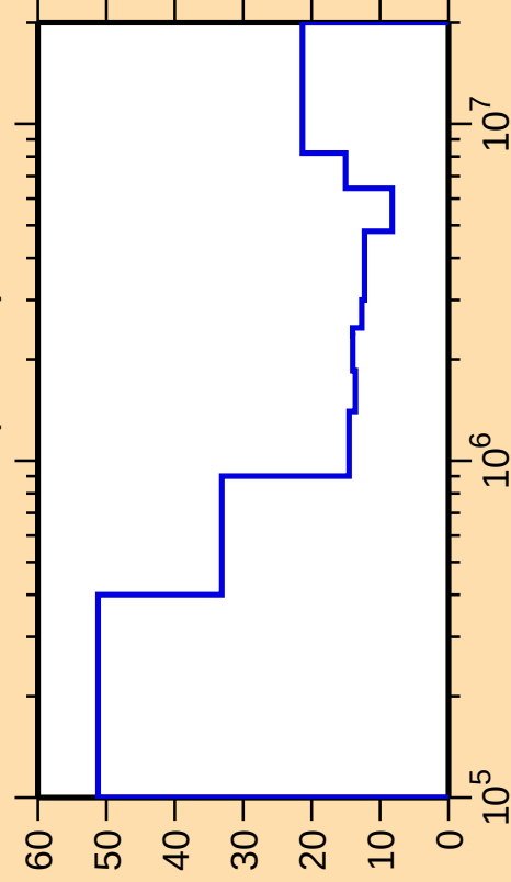
\Delta\sigma/\sigma vs. E for ^{127}\text{Xe}(n,\text{inel.})
