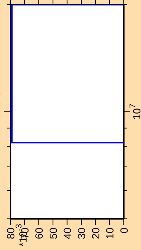
\Delta\sigma/\sigma vs. E for ^{127}\text{Xe}(n,\text{pt})
