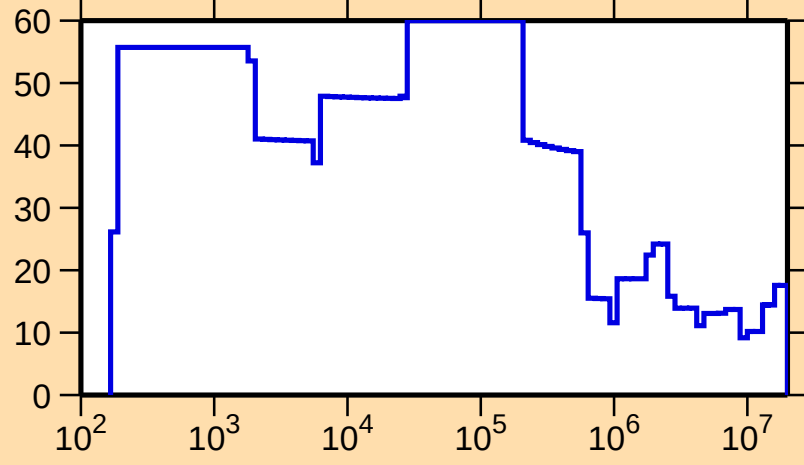
\Delta\sigma/\sigma vs. E for ^{129}\text{Xe}(n,\text{el.})
