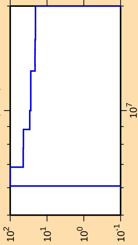
\Delta\sigma/\sigma vs. E for ^{129}\text{Xe}(n,2n)
