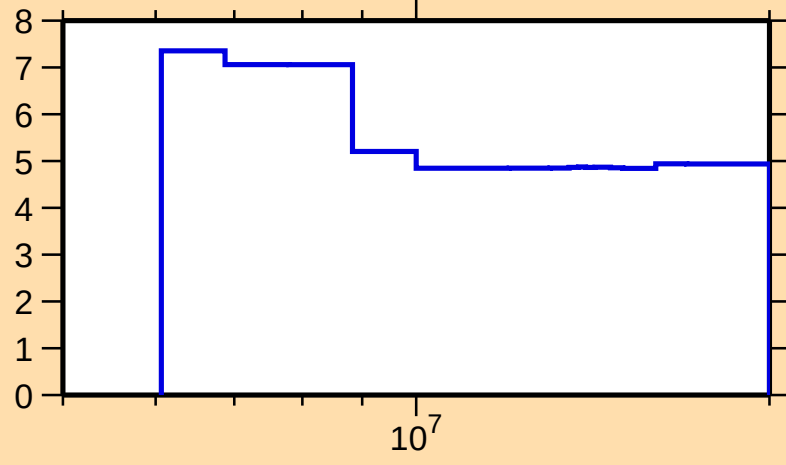
\Delta\sigma/\sigma vs. E for ^{129}\text{Xe}(n,\text{nonel.})
