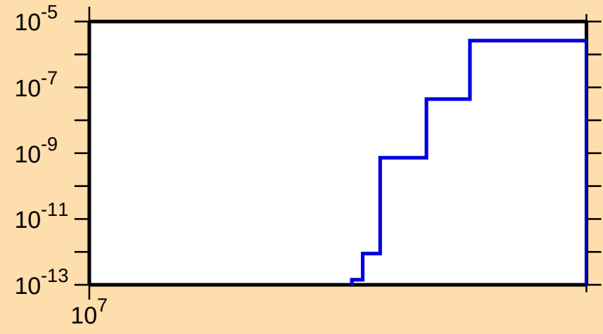
\sigma vs. E for ^{129}\text{Xe}(n,\text{nd})
