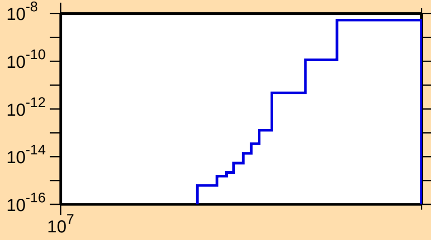
\sigma vs. E for ^{129}\text{Xe}(n,\text{He3})
