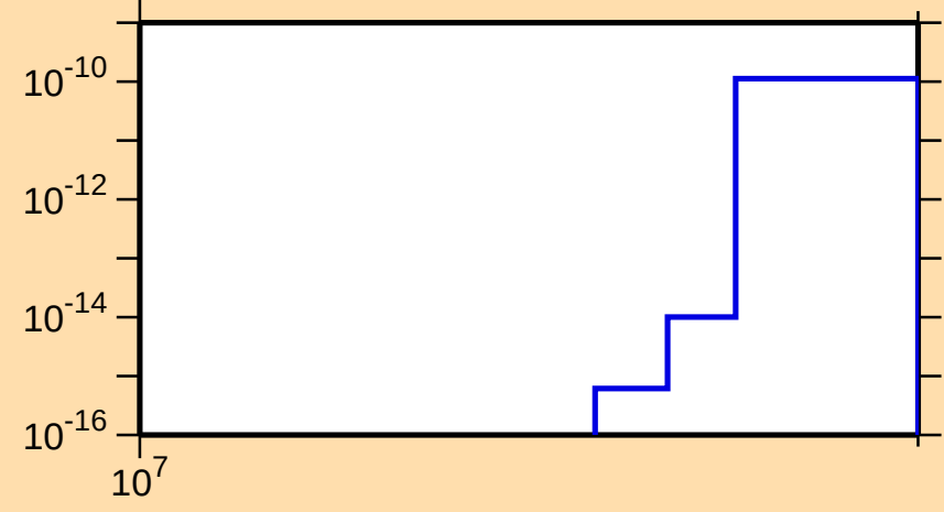
\sigma vs. E for ^{129}\text{Xe}(n,nt)
