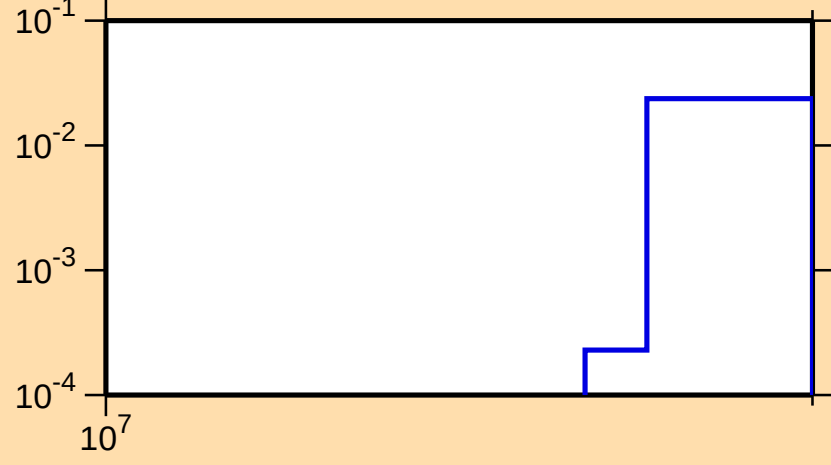
\sigma vs. E for ^{129}\text{Xe}(n,3n)
