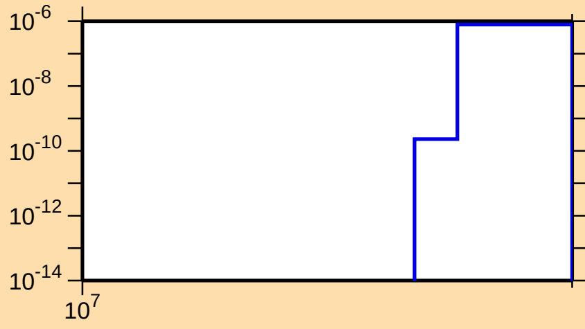
\sigma vs. E for ^{129}\text{Xe}(n,2np)
