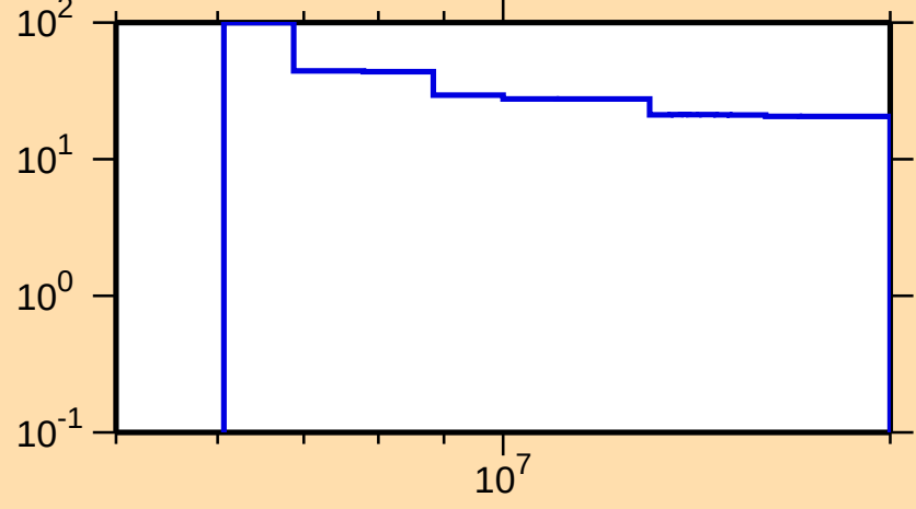
\Delta\sigma/\sigma vs. E for ^{129}\text{Xe}(n,2n)
