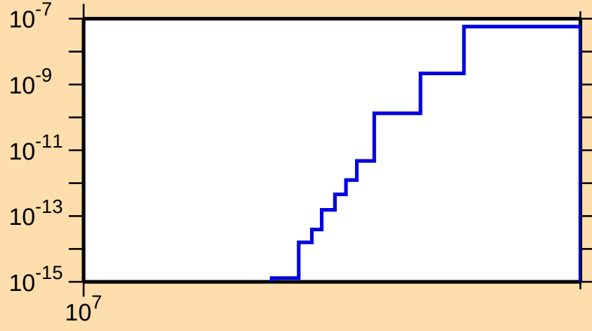
\sigma vs. E for ^{129}\text{Xe}(n,2n\alpha)
