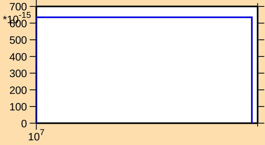
\sigma vs. E for ^{129}\text{Xe}(n,\text{nt})
