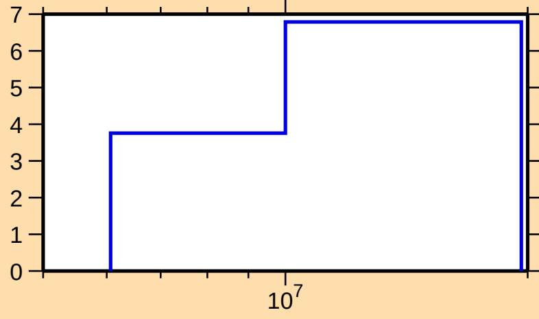
\Delta\sigma/\sigma vs. E for ^{129}\text{Xe}(n,\text{tot.})
