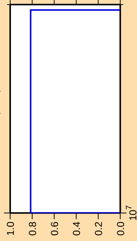
\Delta\sigma/\sigma vs. E for ^{129}\text{Xe}(n,\text{nt})
