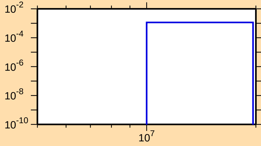
\sigma vs. E for ^{129}\text{Xe}(n,np)
