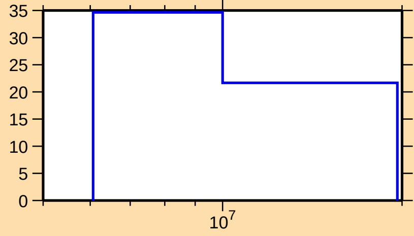
\Delta\sigma/\sigma vs. E for ^{129}\text{Xe}(n,2n)
