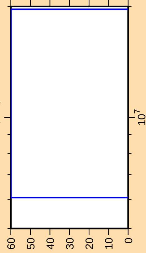
\Delta\sigma/\sigma vs. E for ^{129}\text{Xe}(n,d)
