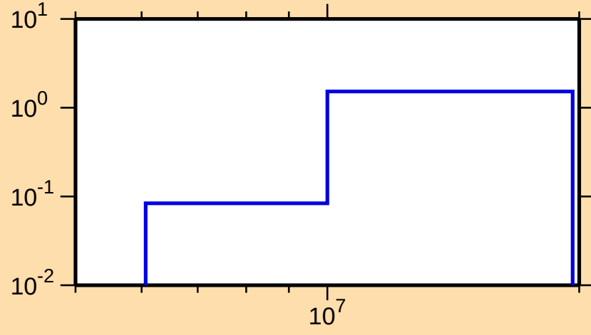
\sigma vs. E for ^{129}\text{Xe}(n,2n)
