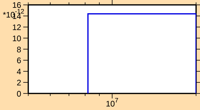
\sigma vs. E for ^{129}\text{Xe}(n,p\alpha)
