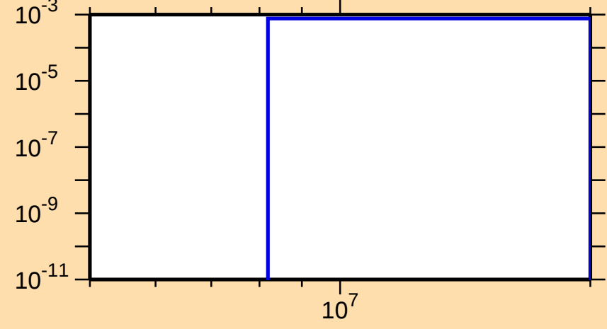
\sigma vs. E for ^{129}\text{Xe}(n,d)
