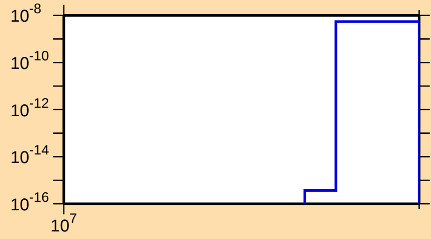
\sigma vs. E for ^{130}\text{Xe}(n,\text{nd})
