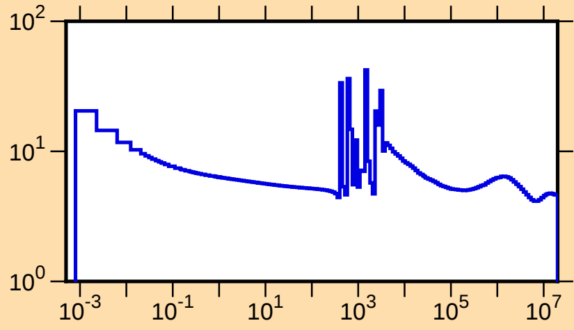
\sigma vs. E for ^{130}\text{Xe}(n,\text{tot.})
