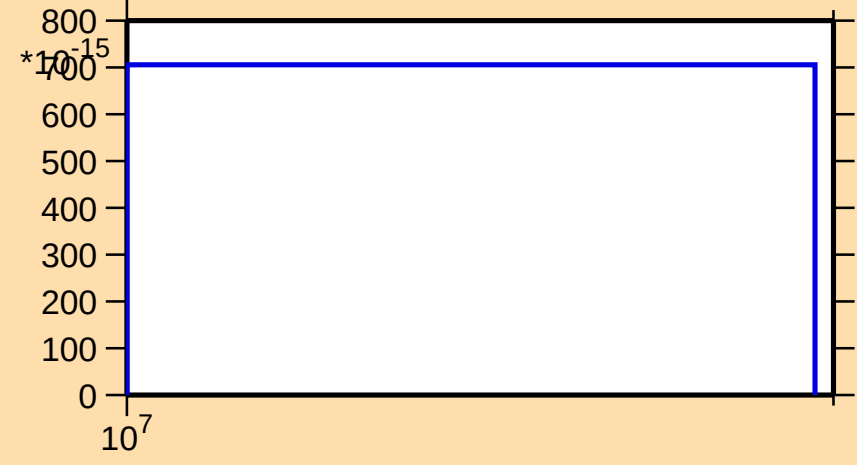
\sigma vs. E for ^{130}\text{Xe}(n,\text{nt})
