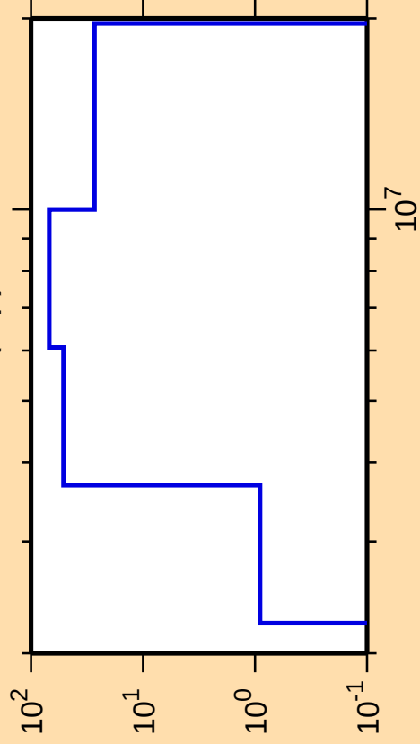
\Delta\sigma/\sigma vs. E for ^{130}\text{Xe}(n,p)
