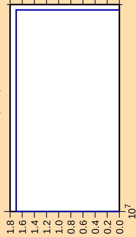
\Delta\sigma/\sigma vs. E for ^{130}\text{Xe}(n,\text{nt})
