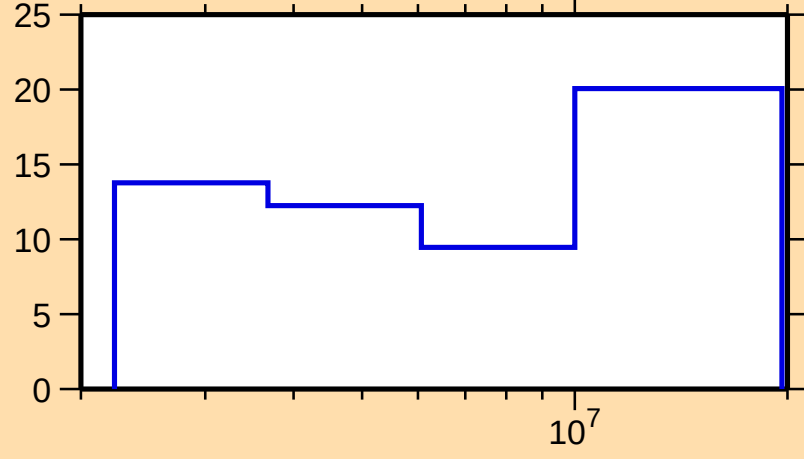
\Delta\sigma/\sigma vs. E for ^{130}\text{Xe}(n,n\text{cont.})
