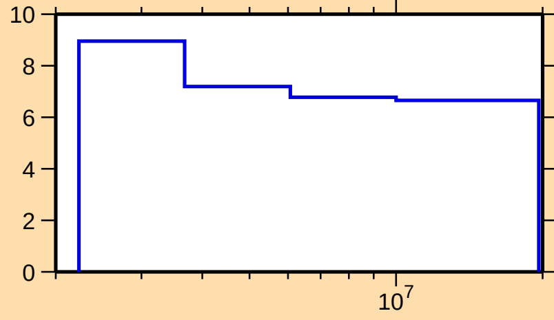
\Delta\sigma/\sigma vs. E for ^{130}\text{Xe}(n,n\text{nonel.})
