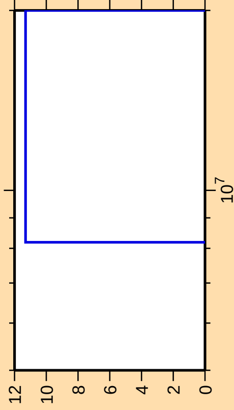
\Delta\sigma/\sigma vs. E for ^{130}\text{Xe}(n,2n)
