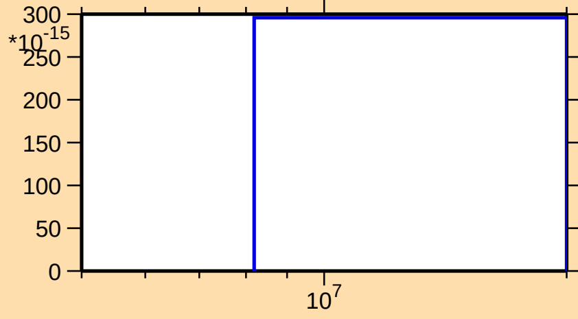
\sigma vs. E for ^{130}\text{Xe}(n,2n\alpha)
