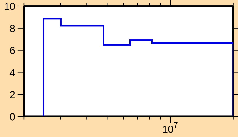
\Delta\sigma/\sigma vs. E for ^{130}\text{Xe}(n,n\text{onel.})
