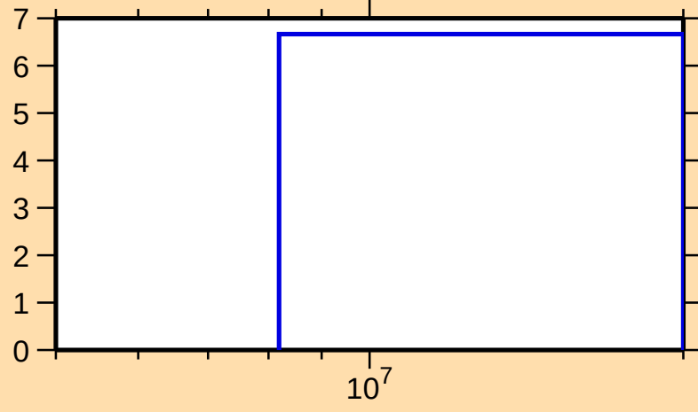
\Delta\sigma/\sigma vs. E for ^{130}\text{Xe}(n,\text{nonel.})
