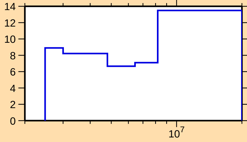
\Delta\sigma/\sigma vs. E for ^{130}\text{Xe}(n,\text{inel.})
