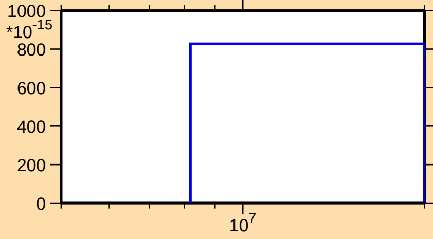
\sigma vs. E for ^{130}\text{Xe}(n,2np)
