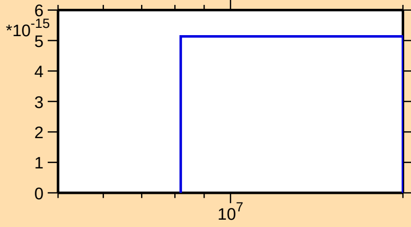
\sigma vs. E for ^{130}\text{Xe}(n,p\alpha)
