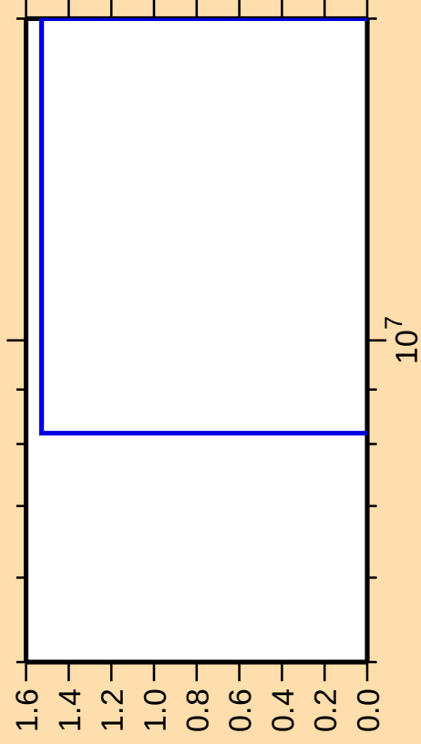
\Delta\sigma/\sigma vs. E for ^{130}\text{Xe}(n,2n\alpha)
