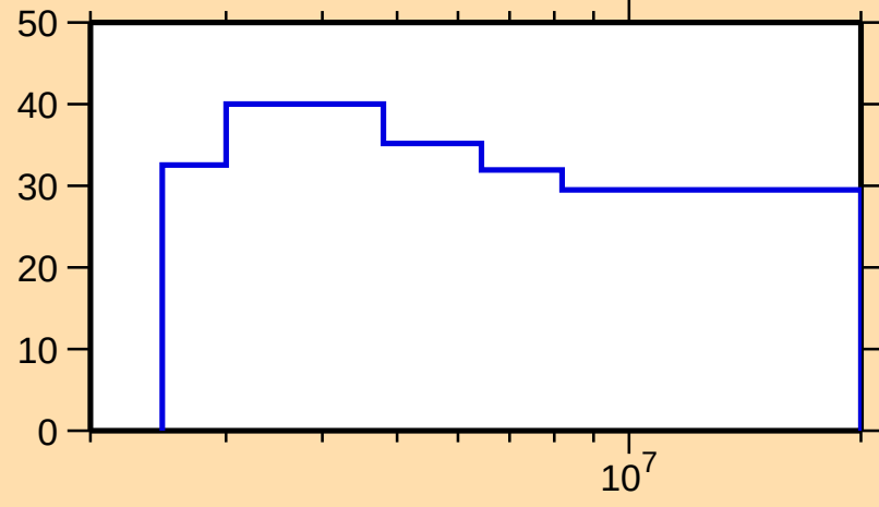
\Delta\sigma/\sigma vs. E for ^{130}\text{Xe}(n, n_1)
