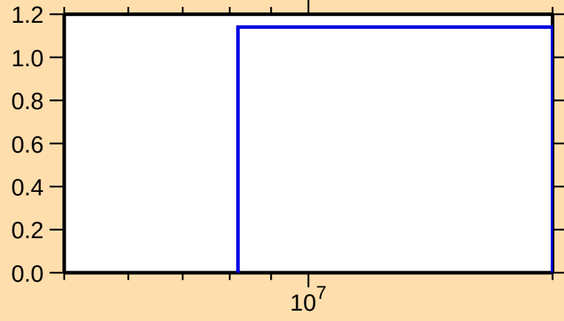
\sigma vs. E for ^{130}\text{Xe}(n,2n)
