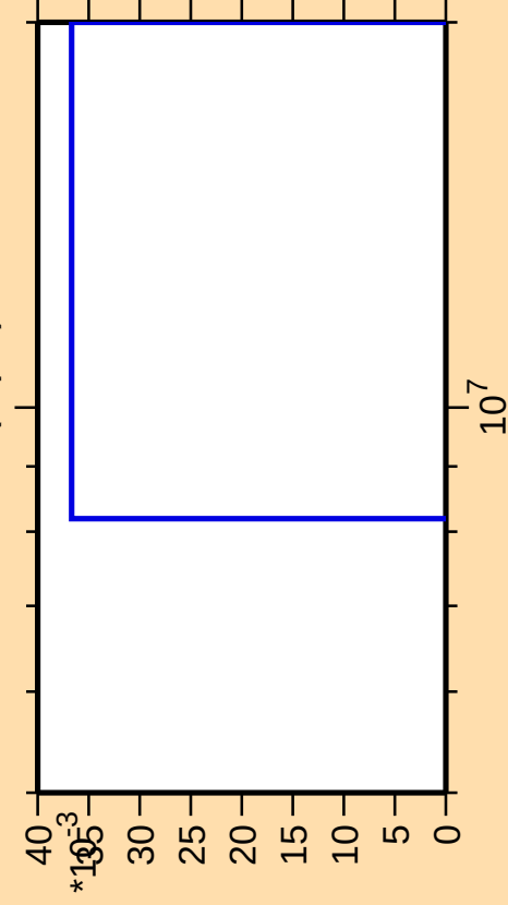
\Delta\sigma/\sigma vs. E for ^{130}\text{Xe}(n,p\alpha)
