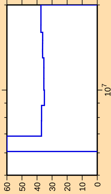
\Delta\sigma/\sigma vs. E for ^{131}\text{Xe}(n,p)
