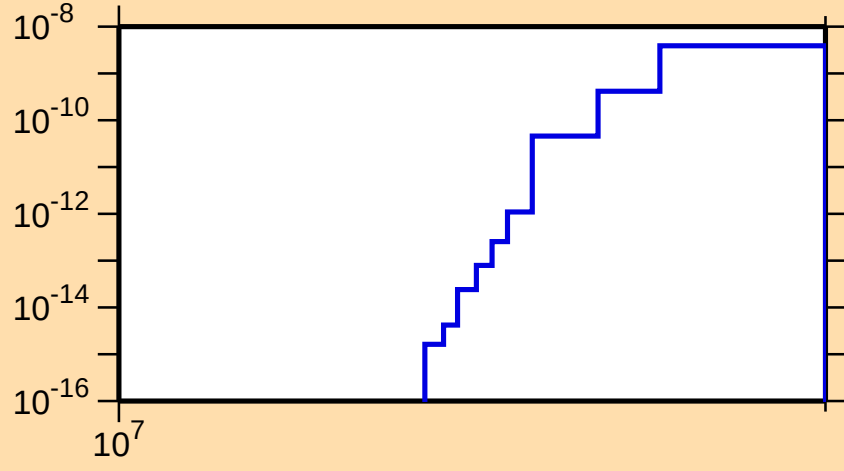
\sigma vs. E for ^{131}\text{Xe}(n,2n\alpha)
