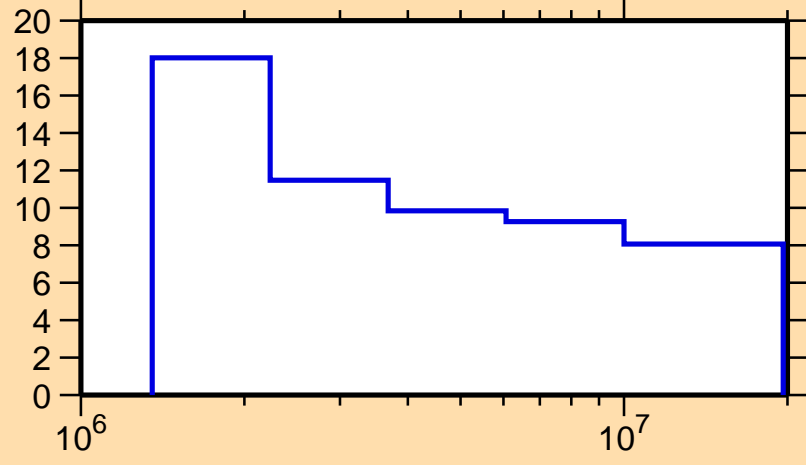
\Delta\sigma/\sigma vs. E for ^{131}\text{Xe}(n,n\text{onel.})
