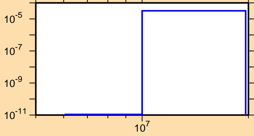
\sigma vs. E for ^{131}\text{Xe}(n,n\alpha)
