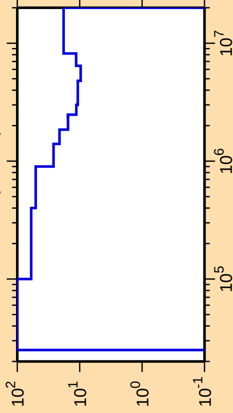
\Delta\sigma/\sigma vs. E for ^{131}\text{Xe}(n,\text{inel.})
