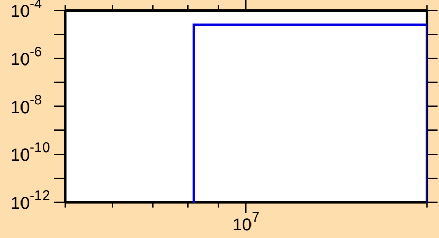
\sigma vs. E for ^{131}\text{Xe}(n,n\alpha)
