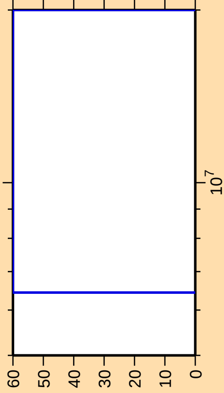
\Delta\sigma/\sigma vs. E for ^{131}\text{Xe}(n,\gamma)
