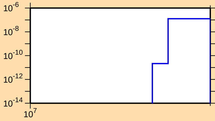
\sigma vs. E for ^{131}\text{Xe}(n,2np)
