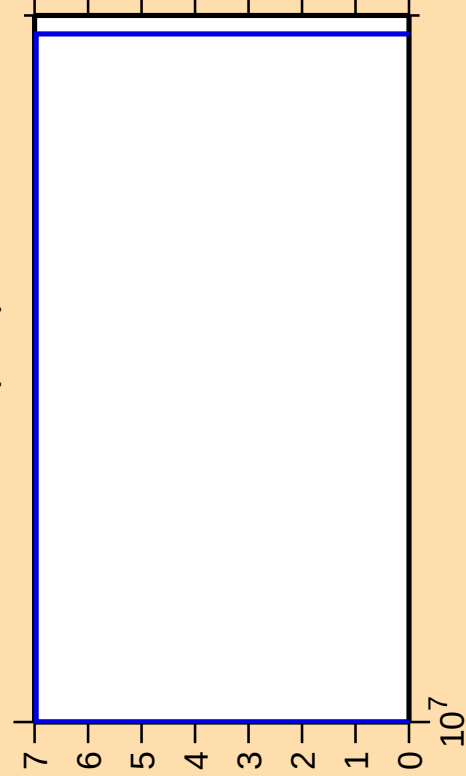
\Delta\sigma/\sigma vs. E for ^{131}\text{Xe}(n,\text{nt})
