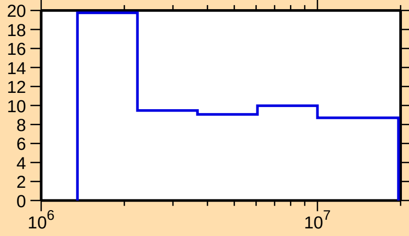
\Delta\sigma/\sigma vs. E for ^{131}\text{Xe}(n,n\text{nonel.})
