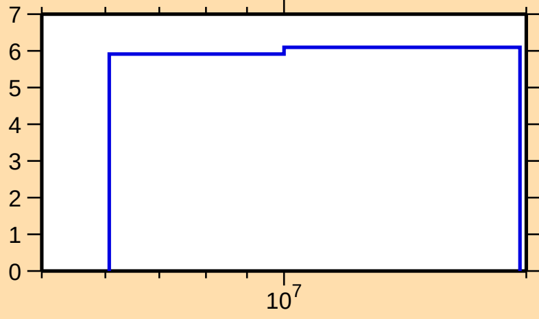
\Delta\sigma/\sigma vs. E for ^{131}\text{Xe}(n,\text{el.})
