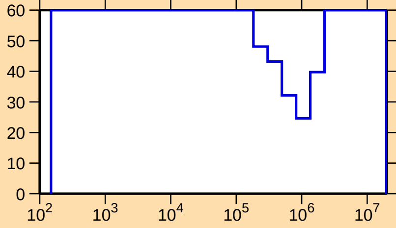
\Delta\sigma/\sigma vs. E for ^{131}\text{Xe}(n,n_1)
