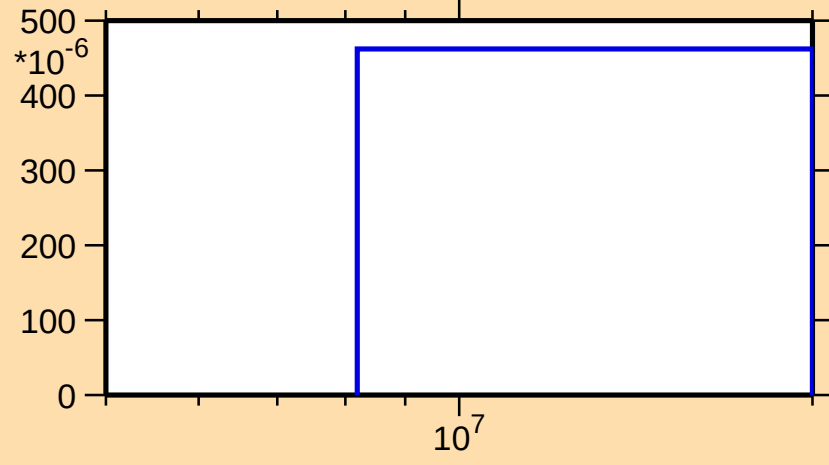
\sigma vs. E for ^{131}\text{Xe}(n,d)
