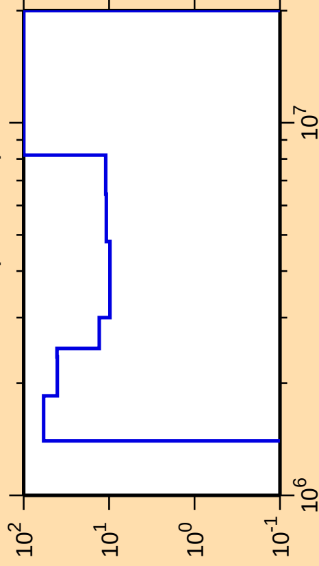
\Delta\sigma/\sigma vs. E for ^{131}\text{Xe}(\text{n},\text{ncont.})
