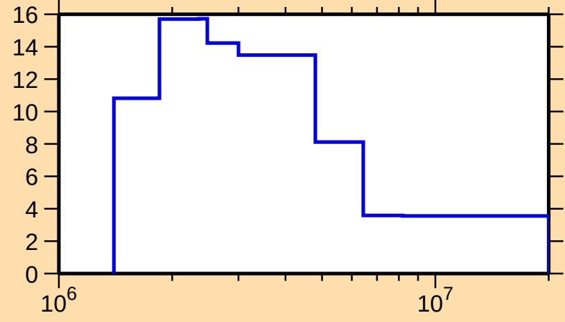
\Delta\sigma/\sigma vs. E for ^{131}\text{Xe}(\text{n},\text{tot.})
