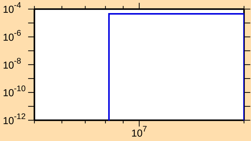
\sigma vs. E for ^{131}\text{Xe}(n,n\alpha)
