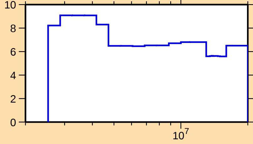
\Delta\sigma/\sigma vs. E for ^{133}\text{Xe}(n,n\text{nonel.})
