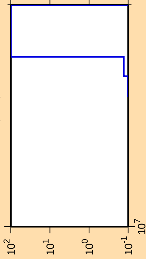
\Delta\sigma/\sigma vs. E for ^{133}\text{Xe}(n,\text{nt})
