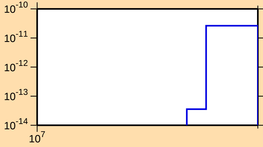
\sigma vs. E for ^{133}\text{Xe}(n,\text{He}3)
