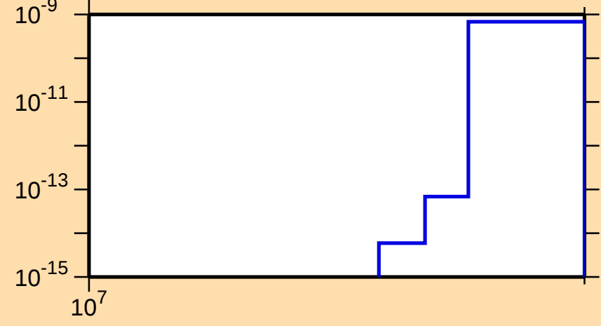
\sigma vs. E for ^{133}\text{Xe}(n,\text{nt})
