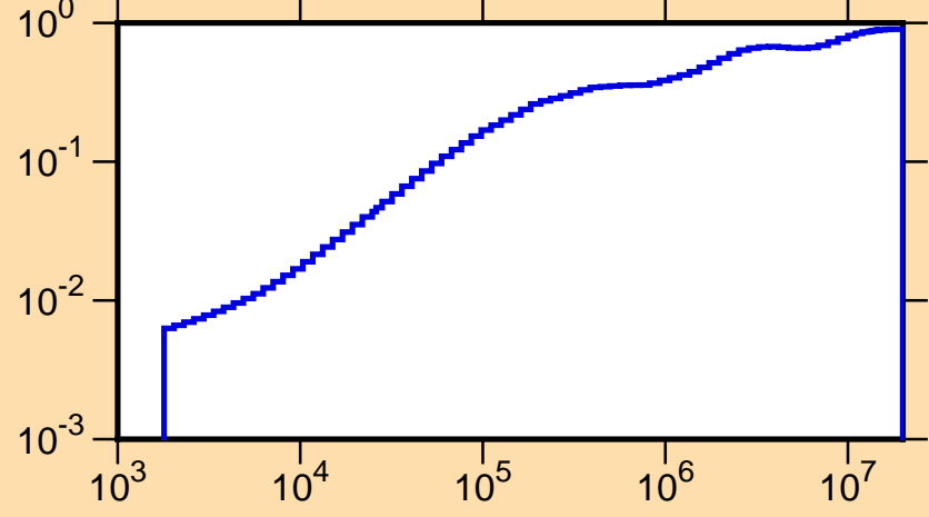
\mu vs. E for ^{134}\text{Xe}(\text{mt251})
