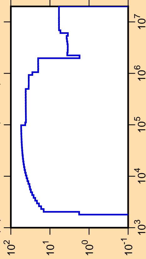
\Delta\mu/\mu vs. E for ^{134}\text{Xe}(\text{mt251})
