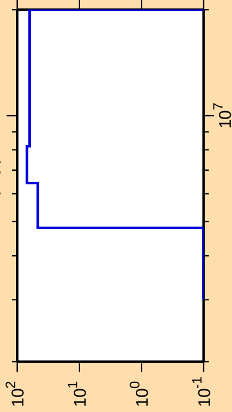
\Delta\sigma/\sigma vs. E for ^{134}\text{Xe}(n,p)
