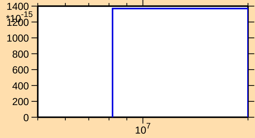
\sigma vs. E for ^{134}\text{Xe}(n,nt)
