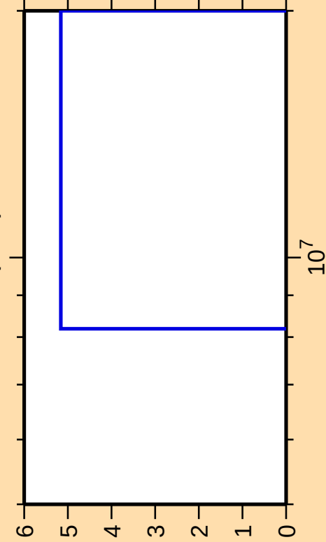
\Delta\sigma/\sigma vs. E for ^{134}\text{Xe}(n,nt)
