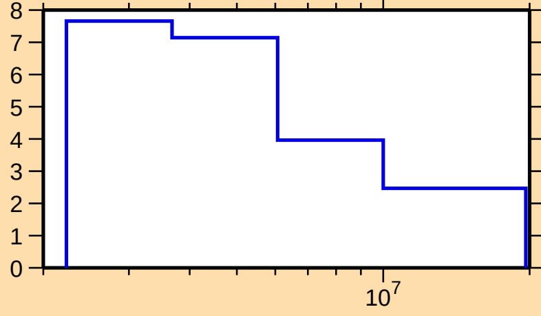
\Delta\sigma/\sigma vs. E for ^{135}\text{Xe}(n,\text{nonel.})
