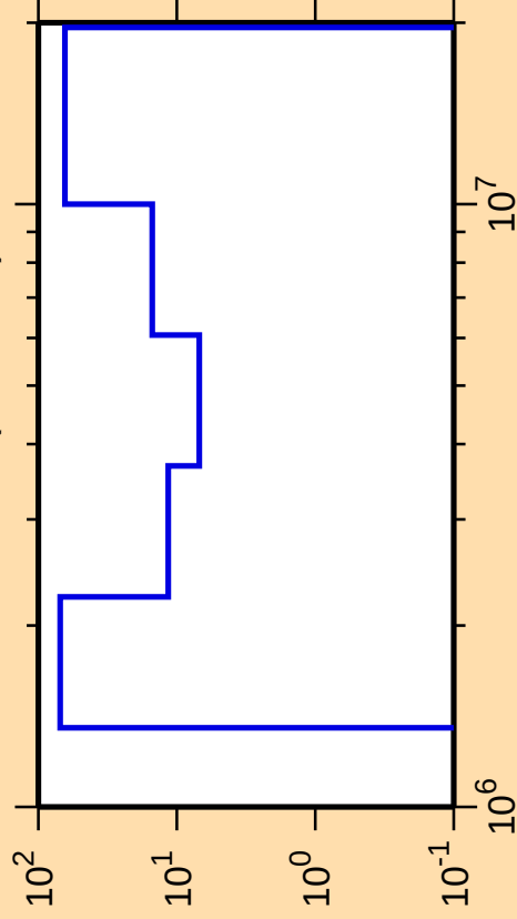
\Delta\sigma/\sigma vs. E for ^{135}\text{Xe}(n,\text{ncont.})
