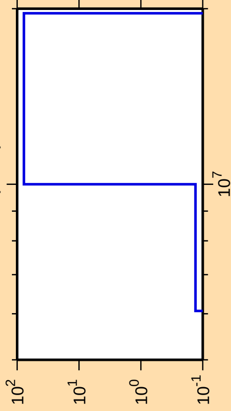
\Delta\sigma/\sigma vs. E for ^{135}\text{Xe}(n,\alpha)
