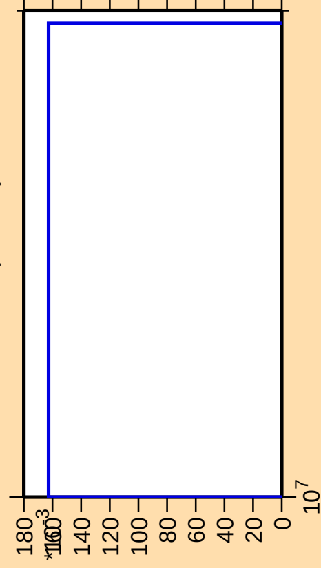
\Delta\sigma/\sigma vs. E for ^{135}\text{Xe}(n,\text{He}3)
