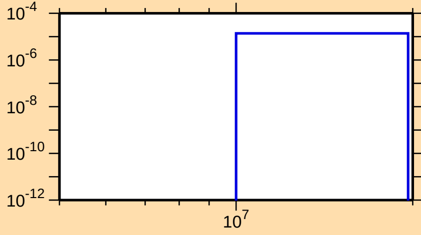
\sigma vs. E for ^{135}\text{Xe}(n,\alpha)
