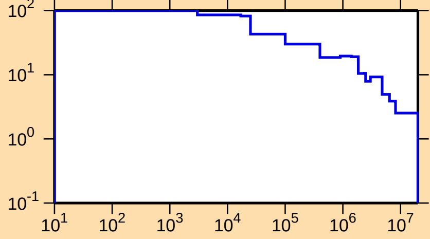
\Delta\sigma/\sigma vs. E for ^{135}\text{Xe}(n,\text{nonel.})
