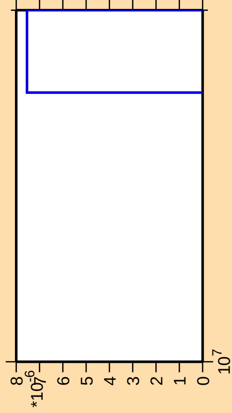
\Delta\sigma/\sigma vs. E for ^{138}\text{Xe}(\text{mt } 42)
