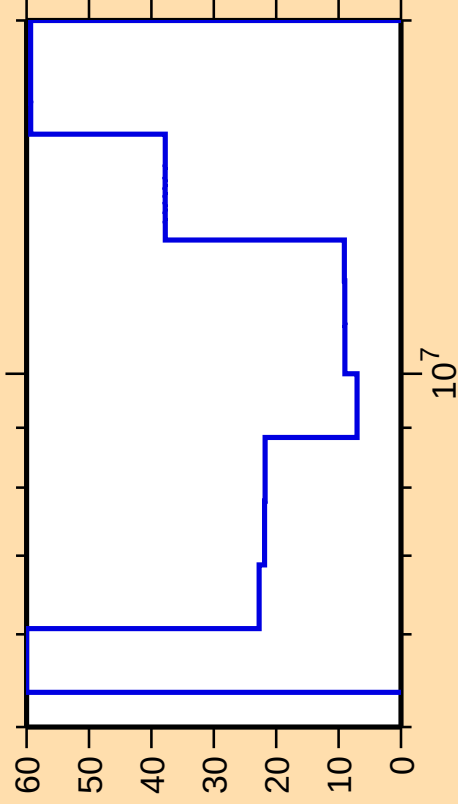
\Delta\sigma/\sigma vs. E for ^{138}\text{Xe}(n,2n)
