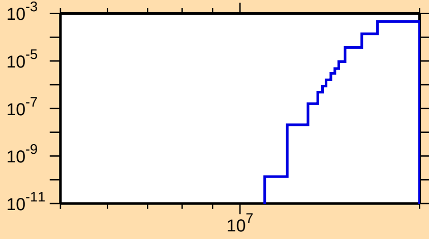
\sigma vs. E for ^{138}\text{Xe}(n,d)
