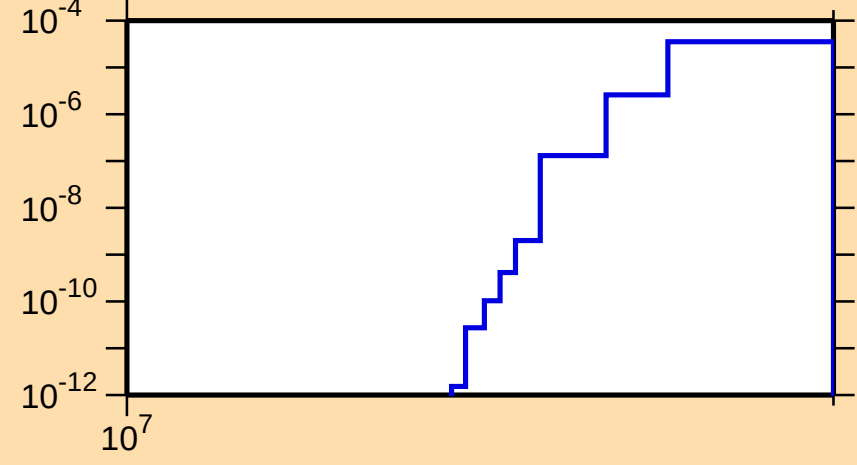
\sigma vs. E for ^{138}\text{Xe}(n,nt)
