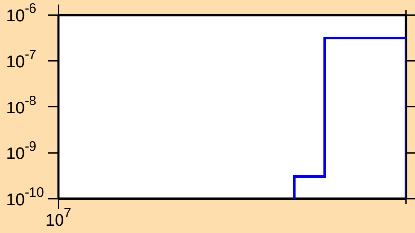
\sigma vs. E for ^{138}\text{Xe}(n,\text{nd})
