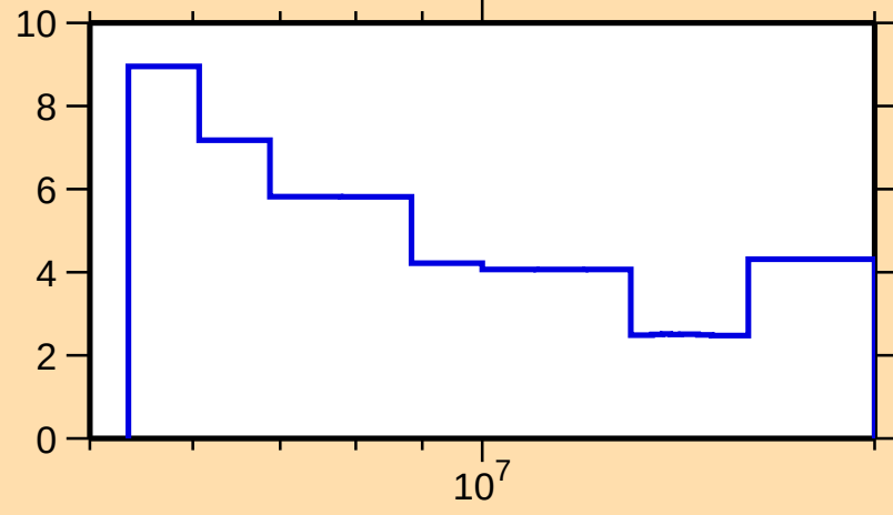
\Delta\sigma/\sigma vs. E for ^{138}\text{Xe}(n,\text{tot.})
