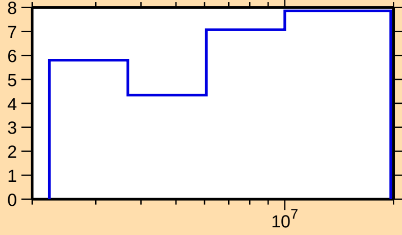
\Delta\sigma/\sigma vs. E for ^{138}\text{Xe}(n,n\text{nonel.})
