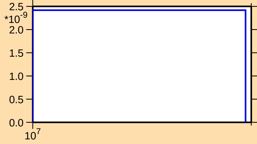
\sigma vs. E for ^{138}\text{Xe}(n,\text{nd})
