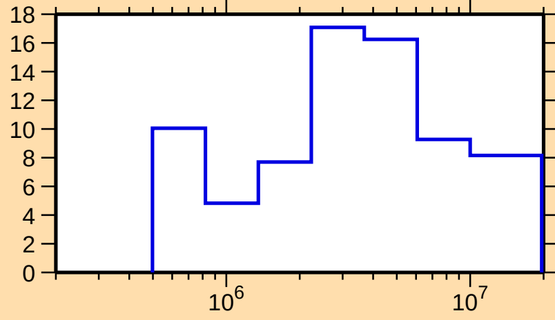
\Delta\sigma/\sigma vs. E for ^{138}\text{Xe}(\text{n,el.})
