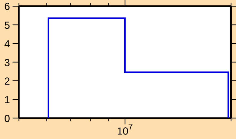
\Delta\sigma/\sigma vs. E for ^{138}\text{Xe}(n,\text{tot.})
