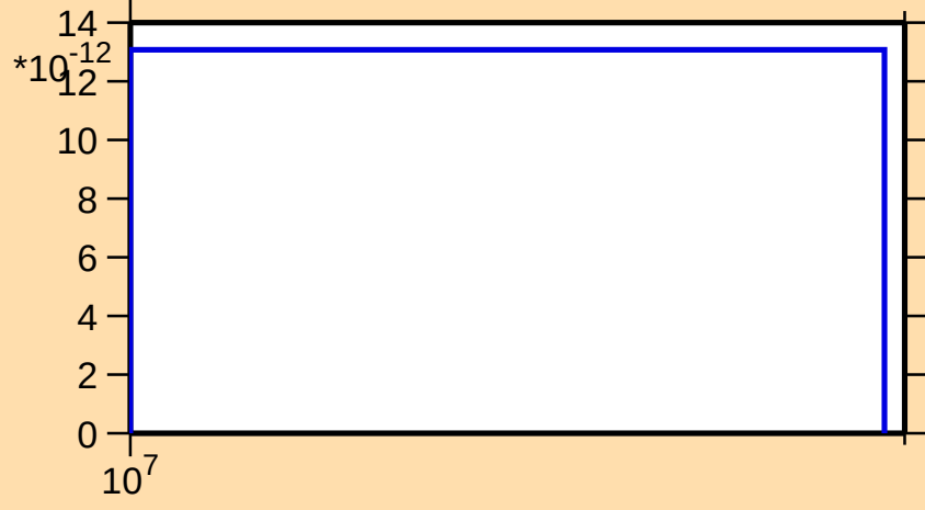
\sigma vs. E for ^{138}\text{Xe}(n,2np)
