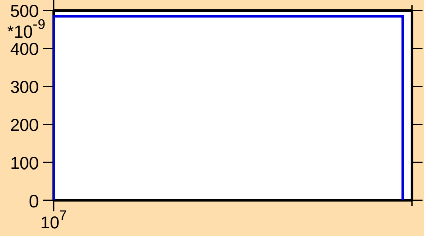
\sigma vs. E for ^{138}\text{Xe}(n,\text{nt})
