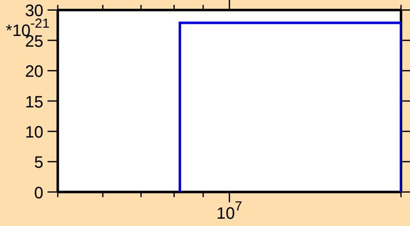
\sigma vs. E for ^{138}\text{Xe}(\text{mt } 42)
