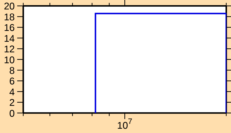
\Delta\sigma/\sigma vs. E for ^{138}\text{Xe}(n,2n)
