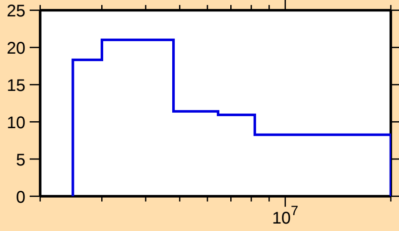
\Delta\sigma/\sigma vs. E for ^{138}\text{Xe}(n,\text{el.})
