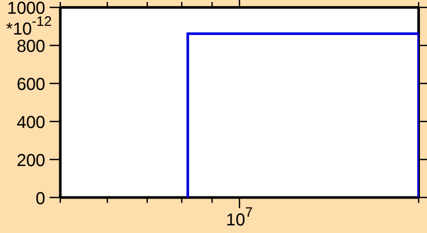
\sigma vs. E for ^{138}\text{Xe}(n,2n\alpha)
