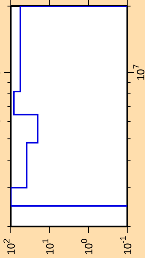
\Delta\sigma/\sigma vs. E for ^{138}\text{Xe}(n,\text{ncont.})
