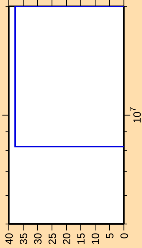
\Delta\sigma/\sigma vs. E for ^{138}\text{Xe}(n,2np)
