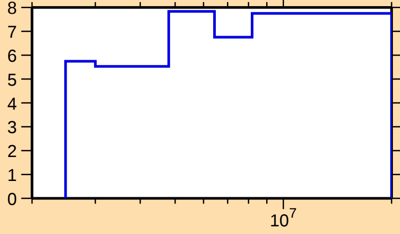
\Delta\sigma/\sigma vs. E for ^{138}\text{Xe}(n,\text{nonel.})
