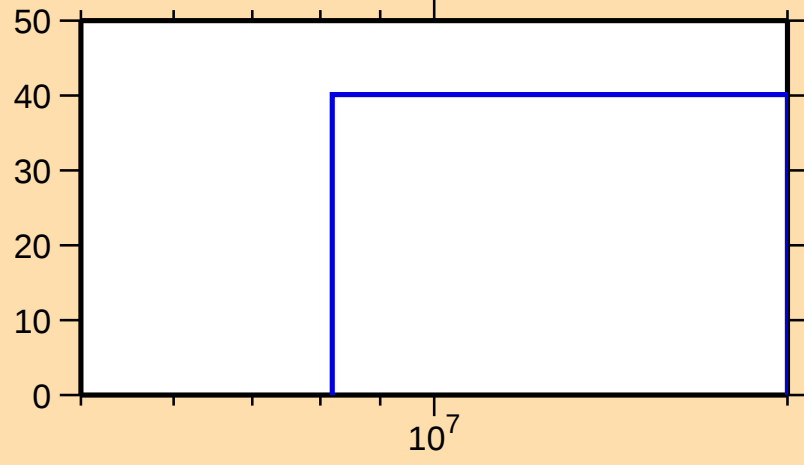
\Delta\sigma/\sigma vs. E for ^{138}\text{Xe}(n,\text{inel.})
