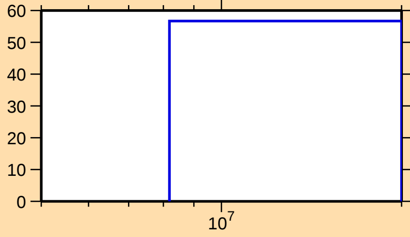
\Delta\sigma/\sigma vs. E for ^{138}\text{Xe}(n,n\text{cont.})
