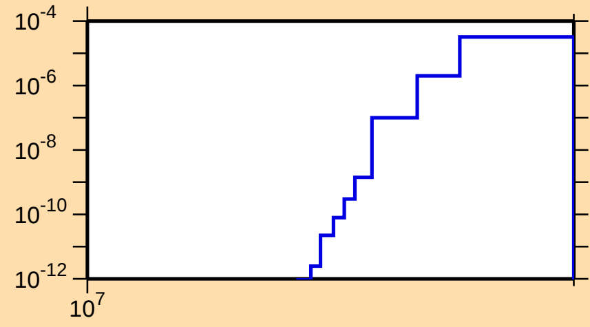
\sigma vs. E for ^{139}\text{Xe}(n,\text{nt})
