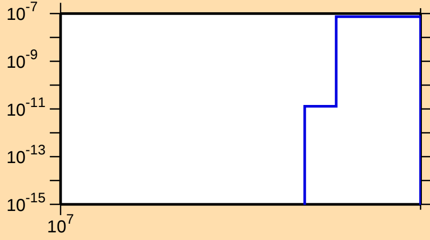
\sigma vs. E for ^{139}\text{Xe}(n,2np)
