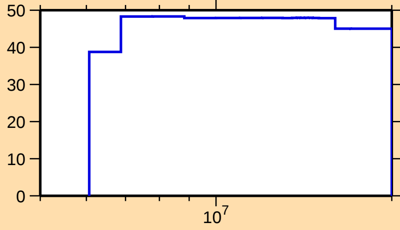
\Delta\sigma/\sigma vs. E for ^{139}\text{Xe}(n,n_1)
