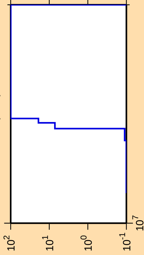
\Delta\sigma/\sigma vs. E for ^{139}\text{Xe}(n,\text{nt})
