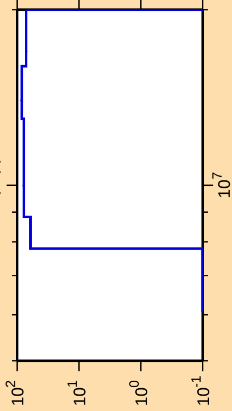
\Delta\sigma/\sigma vs. E for ^{139}\text{Xe}(n,p)
