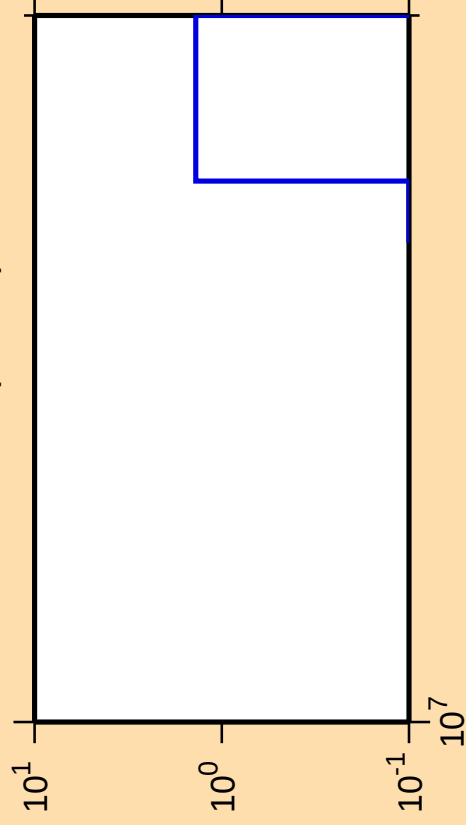
\Delta\sigma/\sigma vs. E for ^{139}\text{Xe}(n,3n\alpha)
