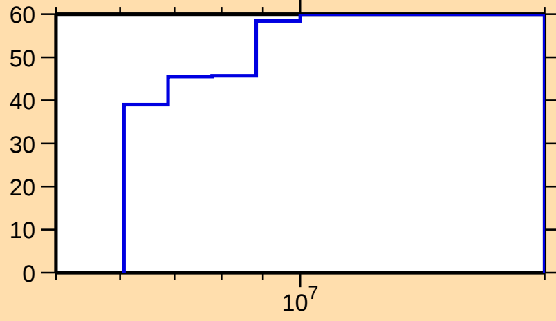
\Delta\sigma/\sigma vs. E for ^{139}\text{Xe}(n,n\text{cont.})
