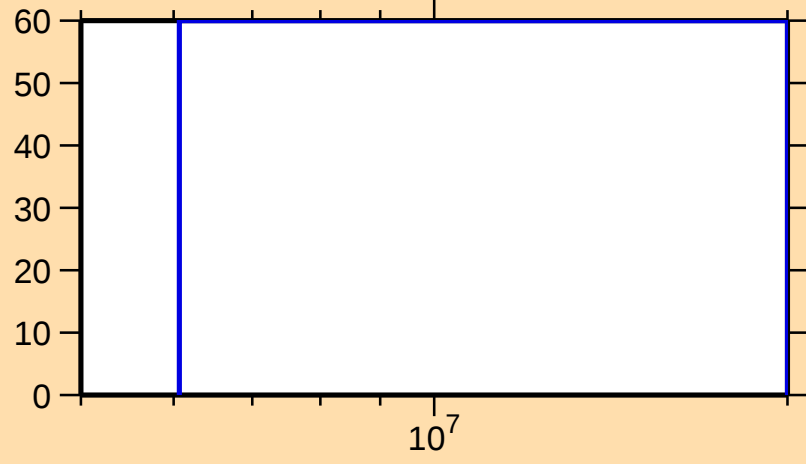
\Delta\sigma/\sigma vs. E for ^{139}\text{Xe}(n,\gamma)
