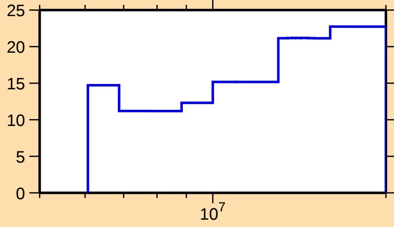
\Delta\sigma/\sigma vs. E for ^{139}\text{Xe}(n,\text{el.})
