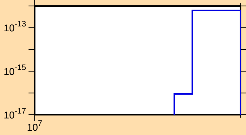
\sigma vs. E for ^{139}\text{Xe}(n,3n\alpha)
