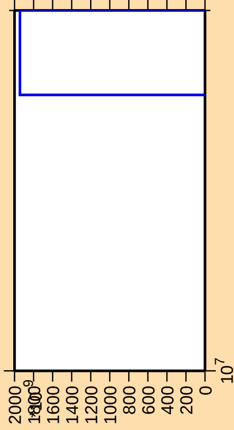
\Delta\sigma/\sigma vs. E for ^{139}\text{Xe}(\text{mt } 42)
