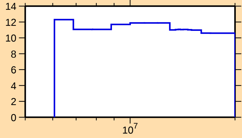
\Delta\sigma/\sigma vs. E for ^{139}\text{Xe}(n,\text{nonel.})
