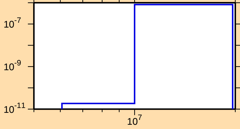
\sigma vs. E for ^{139}\text{Xe}(n,2n\alpha)
