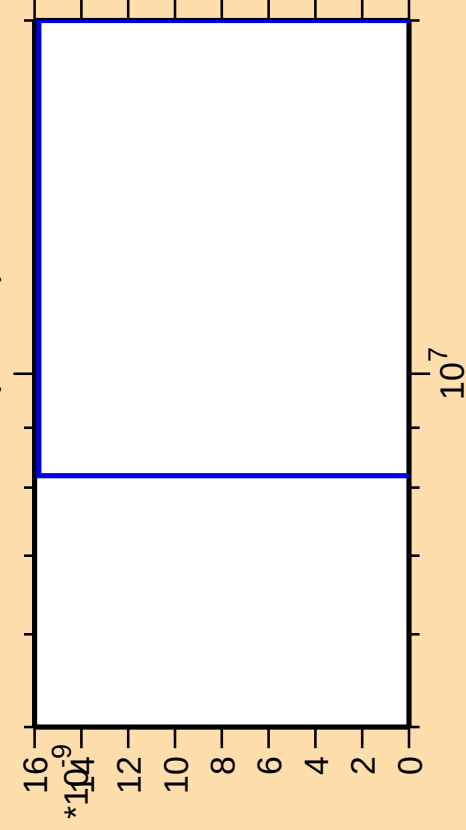
\Delta\sigma/\sigma vs. E for ^{139}\text{Xe}(\text{mt } 42)
