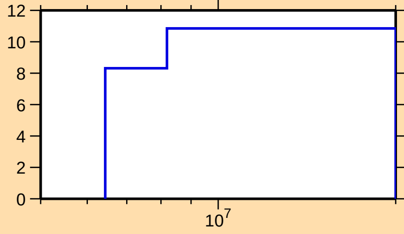
\Delta\sigma/\sigma vs. E for ^{139}\text{Xe}(n,\text{tot.})
