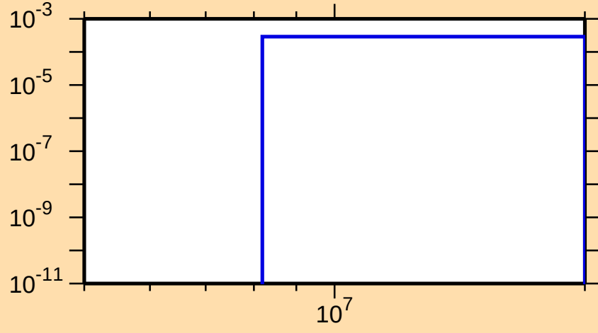
\sigma vs. E for ^{139}\text{Xe}(n,p)
