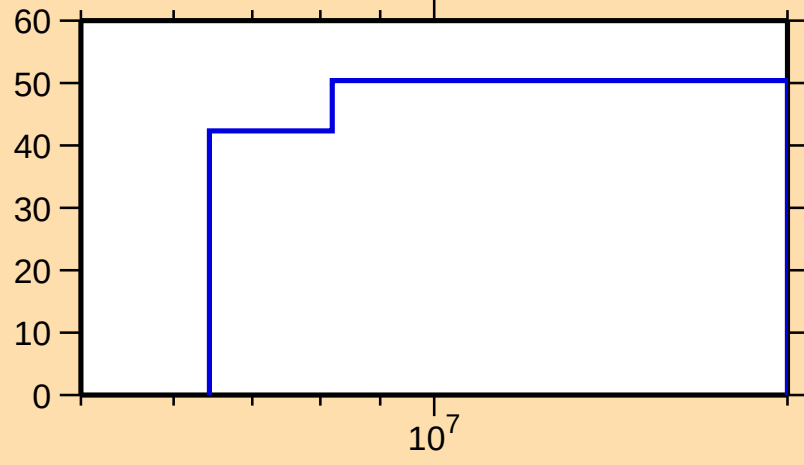
\Delta\sigma/\sigma vs. E for ^{139}\text{Xe}(n,\text{inel.})
