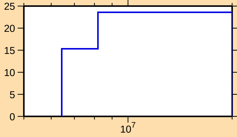
\Delta\sigma/\sigma vs. E for ^{139}\text{Xe}(n,2n)
