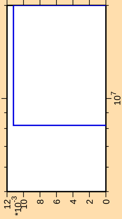
\Delta\sigma/\sigma vs. E for ^{139}\text{Xe}(n,3n\alpha)
