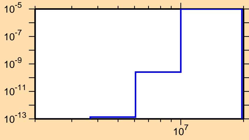
\sigma vs. E for ^{142}\text{Xe}(n,\alpha)
