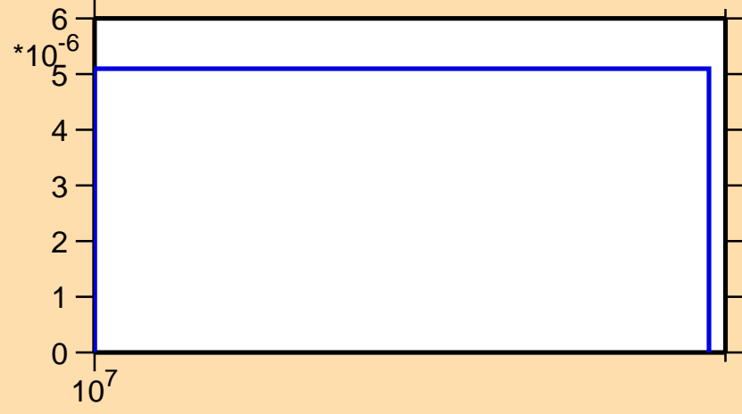
\sigma vs. E for ^{142}\text{Xe}(n,p)
