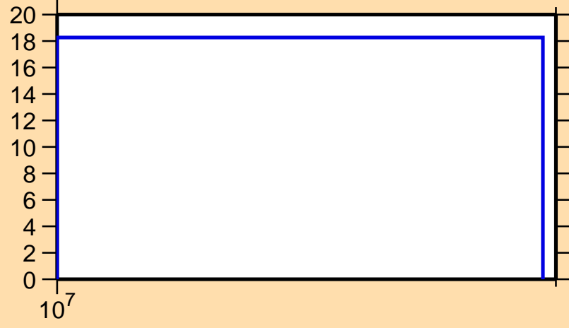
\Delta\sigma/\sigma vs. E for ^{142}\text{Xe}(n,el.)
