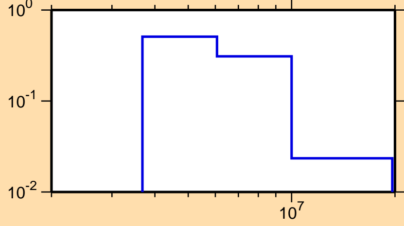
\sigma vs. E for ^{142}\text{Xe}(n,n\text{cont.})
