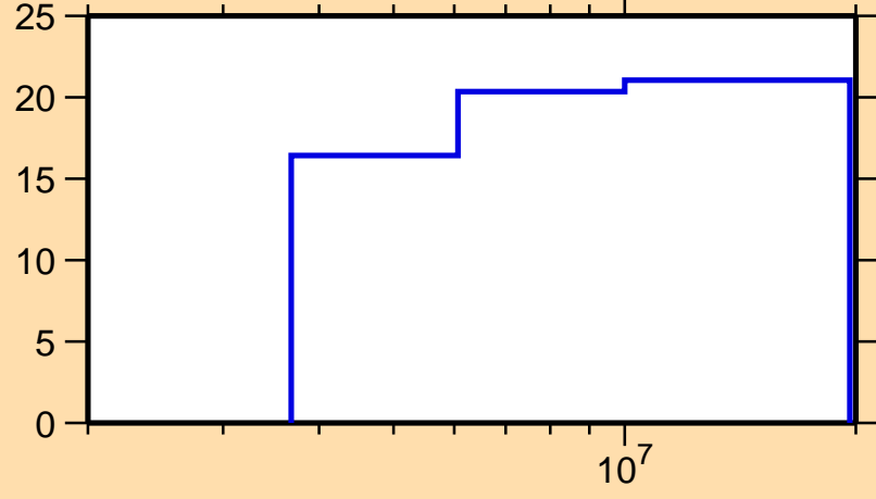
\Delta\sigma/\sigma vs. E for ^{142}\text{Xe}(n,n\text{nonel.})
