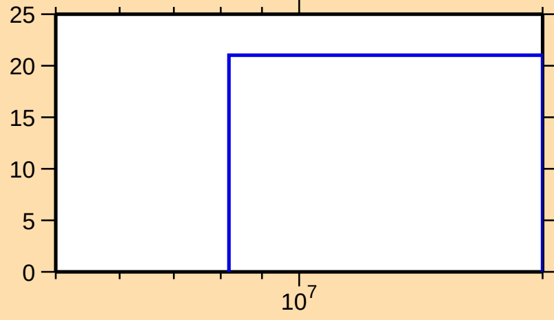
\Delta\sigma/\sigma vs. E for ^{142}\text{Xe}(n,\text{nonel.})
