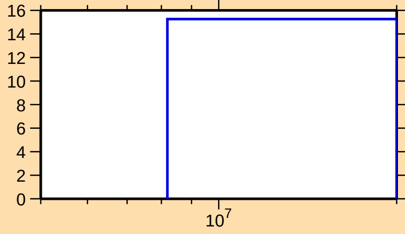
\Delta\sigma/\sigma vs. E for ^{142}\text{Xe}(n,\text{el.})
