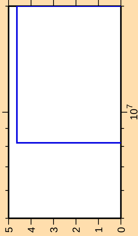
\Delta\sigma/\sigma vs. E for ^{142}\text{Xe}(n,3n\alpha)
