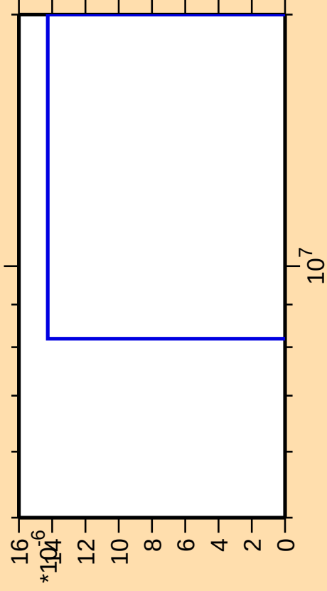
\Delta\sigma/\sigma vs. E for ^{142}\text{Xe}(\text{mt 11})
