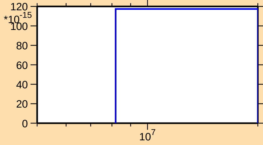
\sigma vs. E for ^{142}\text{Xe}(n,2np)
