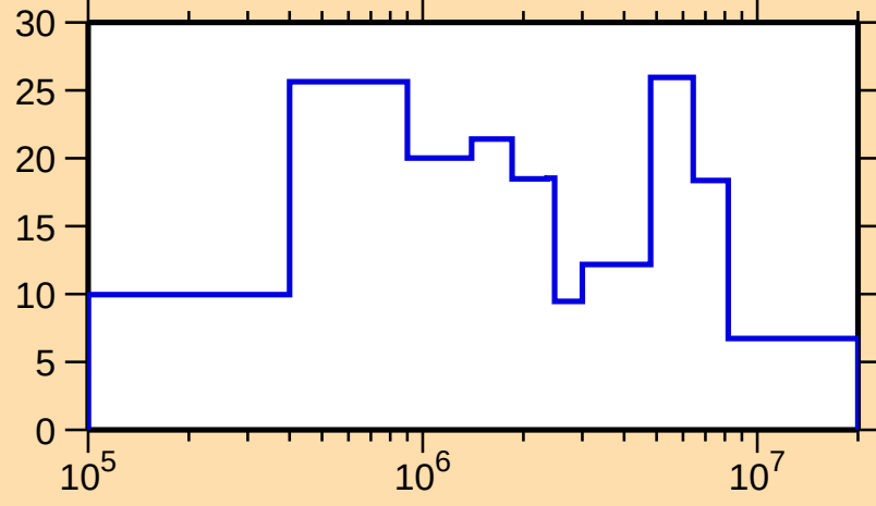
\Delta\sigma/\sigma vs. E for ^{142}\text{Xe}(n,\text{tot.})
