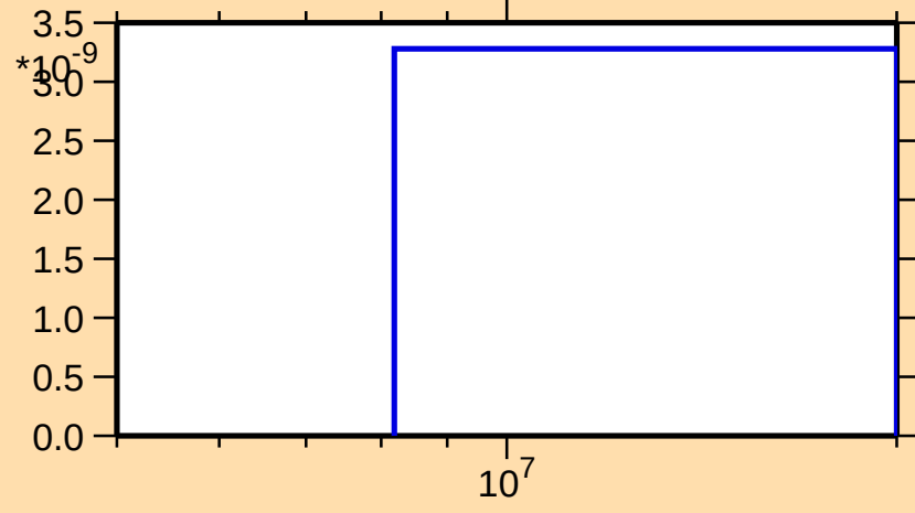
\sigma vs. E for ^{142}\text{Xe}(n,2n\alpha)
