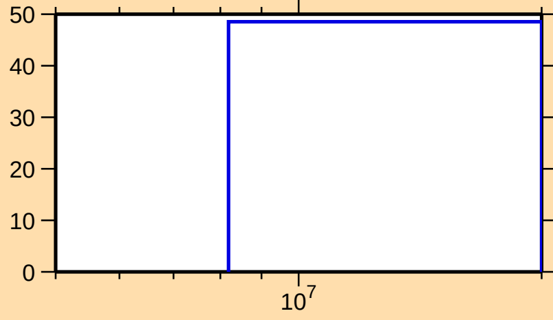
\Delta\sigma/\sigma vs. E for ^{142}\text{Xe}(n,2n)
