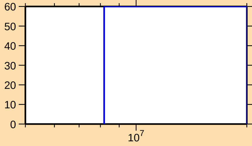
\Delta\sigma/\sigma vs. E for ^{142}\text{Xe}(n,\text{inel.})
