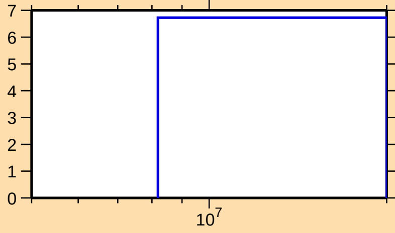
\Delta\sigma/\sigma vs. E for ^{142}\text{Xe}(n,\text{tot.})
