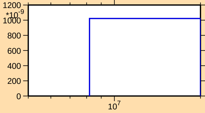
\sigma vs. E for ^{142}\text{Xe}(n,d)
