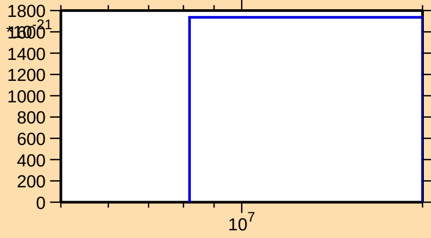
\sigma vs. E for ^{142}\text{Xe}(\text{mt 11})
