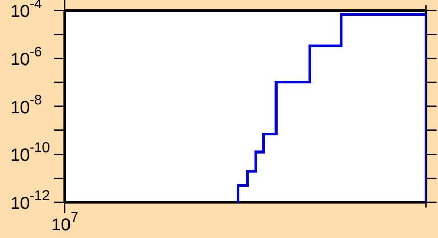
\sigma vs. E for ^{80}\text{Y}(n,\text{pt})
