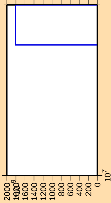
\Delta\sigma/\sigma vs. E for ^{80}\text{Y}(\text{n},\text{nt})
