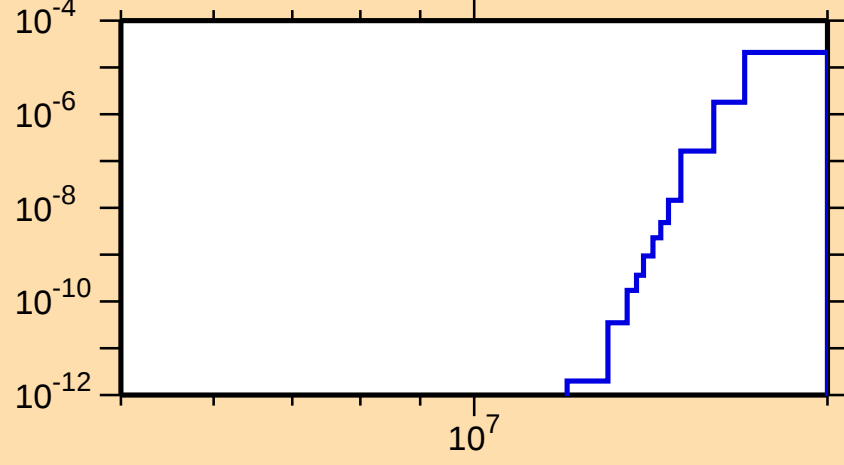
\sigma vs. E for ^{80}\text{Y}(\text{mt } 45)
