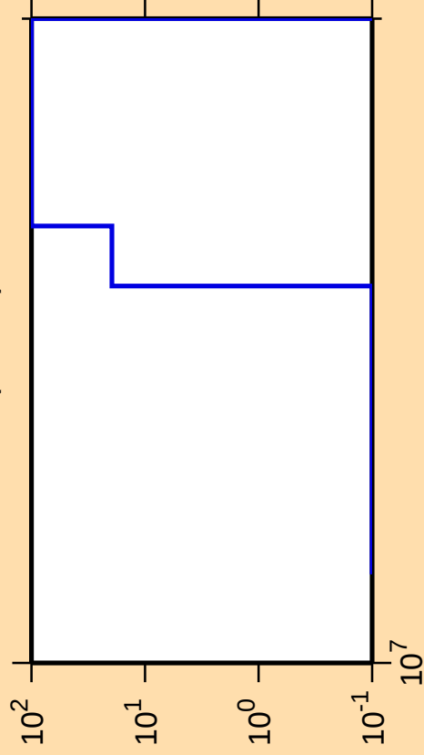
\Delta\sigma/\sigma vs. E for ^{80}\text{Y}(\text{mt } 34)
