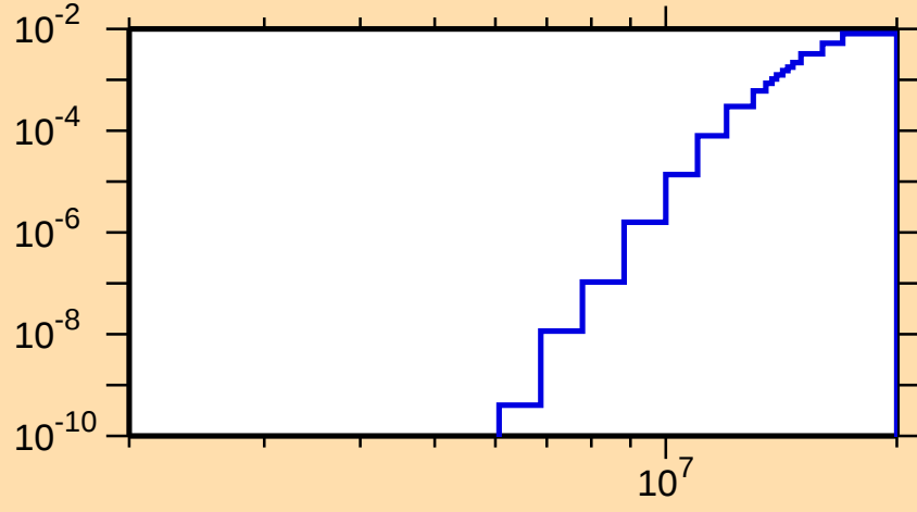
\sigma vs. E for ^{80}\text{Y}(n,\text{He}3)
