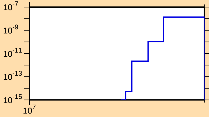
\sigma vs. E for ^{80}\text{Y}(\text{mt } 34)
