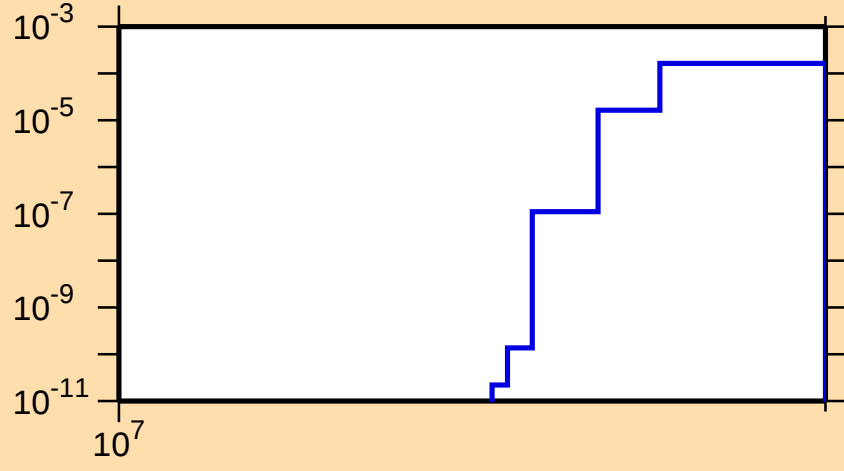
\sigma vs. E for ^{80}\text{Y}(n,2np)
