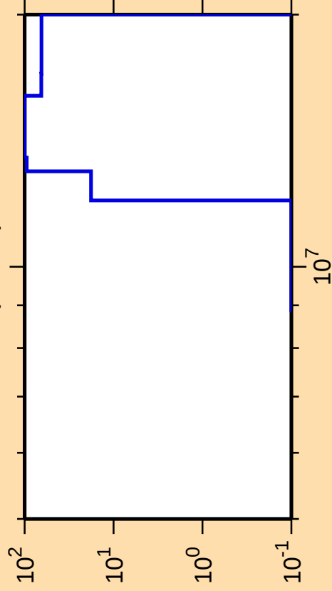
\Delta\sigma/\sigma vs. E for ^{80}\text{Y}(\text{mt } 45)
