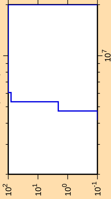
\Delta\sigma/\sigma vs. E for ^{80}\text{Y}(n,\text{He}3)
