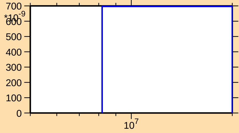
\sigma vs. E for ^{80}\text{Y}(\text{n},\text{pt})
