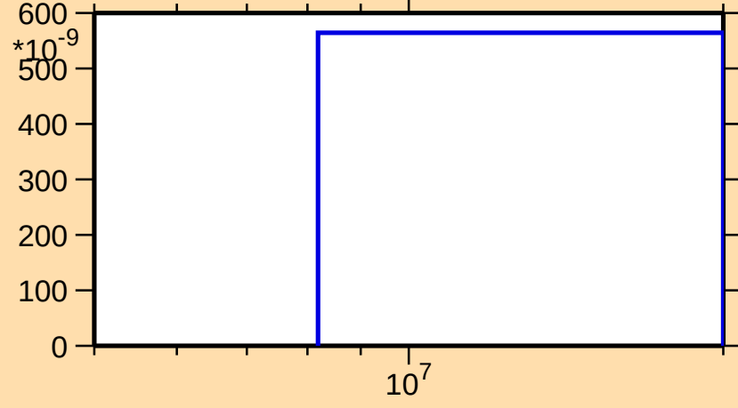
\sigma vs. E for ^{80}\text{Y}(n,\text{nd})
