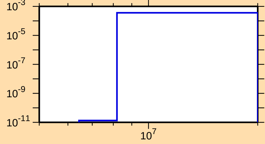
\sigma vs. E for ^{80}\text{Y}(n,n\alpha)
