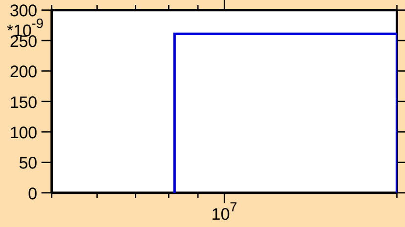
\sigma vs. E for ^{80}\text{Y}(\text{mt } 45)
