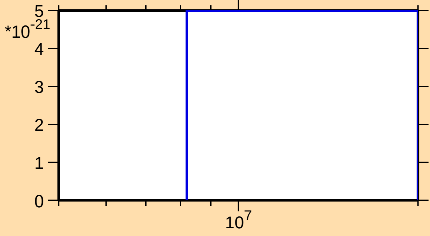
\sigma vs. E for ^{80}\text{Y}(n,nt)
