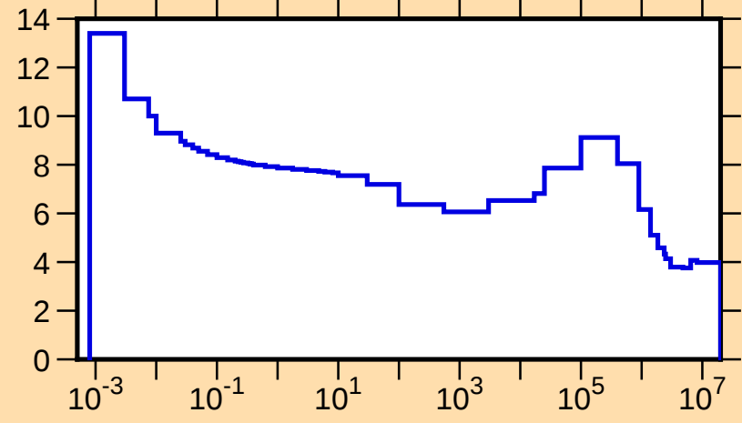
\sigma vs. E for ^{89}\text{Y}(n,\text{tot.})
