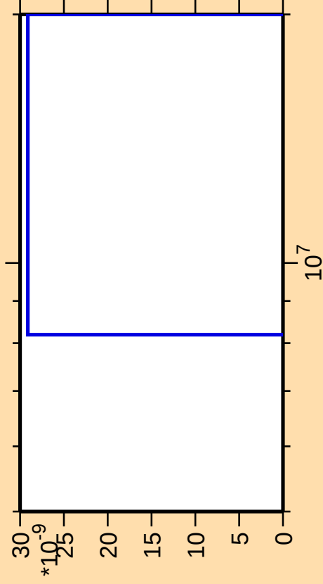
\Delta\sigma/\sigma vs. E for ^{89}\text{Y}(n,2n\alpha)
