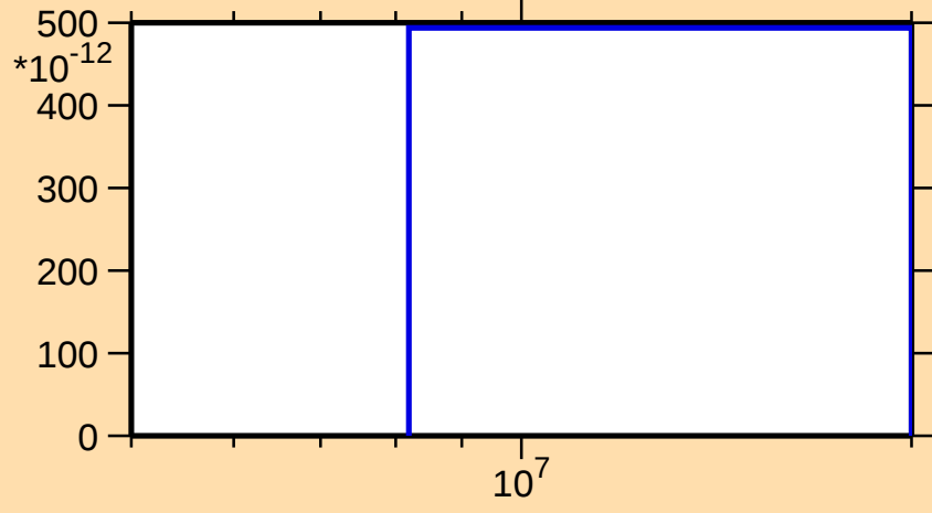
\sigma vs. E for ^{89}\text{Y}(n,\text{nd})
