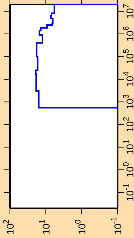
\Delta\sigma/\sigma vs. E for ^{89}\text{Y}(n,\text{nonel.})
