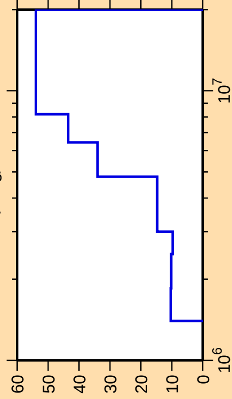
\Delta\sigma/\sigma vs. E for ^{89}\text{Y}(n,n_3)
