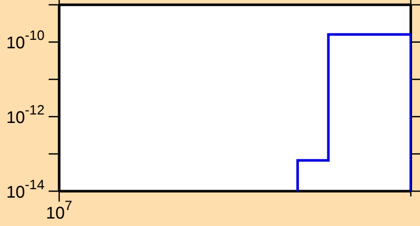
\sigma vs. E for ^{91}\text{Y}(n,\text{He}3)
