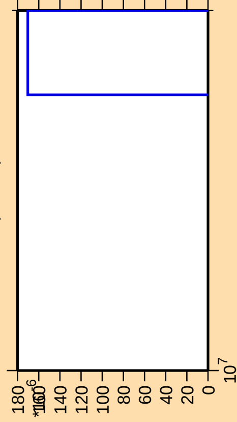
\Delta\sigma/\sigma vs. E for ^{91}\text{Y} (mt 34)
