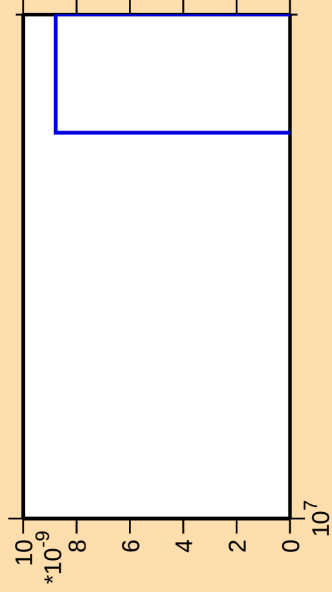
\Delta\sigma/\sigma vs. E for ^{91}\text{Y}(\text{mt 11})
