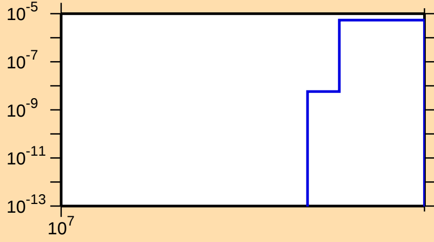
\sigma vs. E for ^{91}\text{Y}(n,2np)
