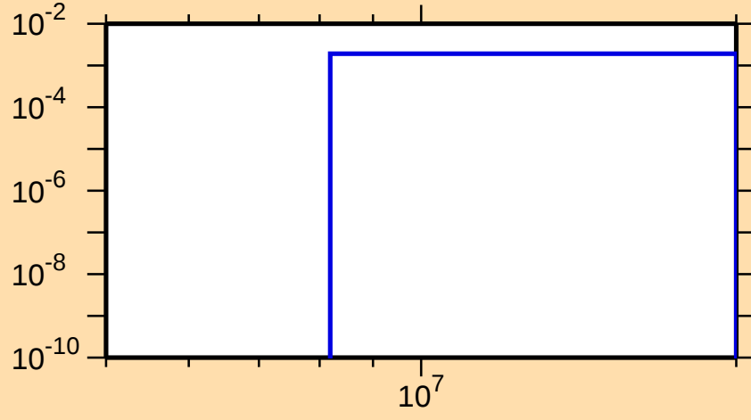
\sigma vs. E for ^{91}\text{Y}(n,np)
