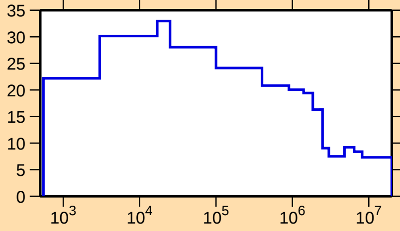
\Delta\sigma/\sigma vs. E for ^{91}\text{Y}(\text{n,nonel.})
