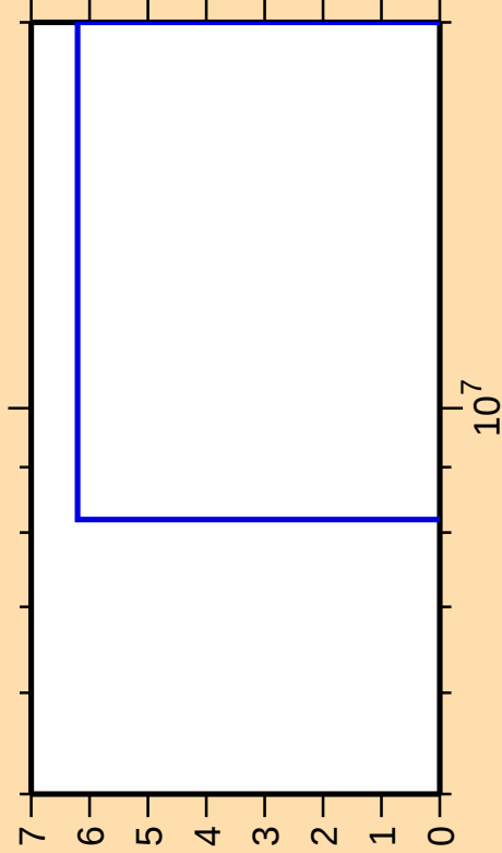
\Delta\sigma/\sigma vs. E for ^{91}\text{Y}(n,\text{He}3)
