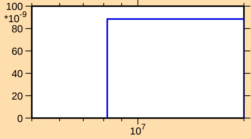
\sigma vs. E for ^{91}\text{Y}(n,nt)
