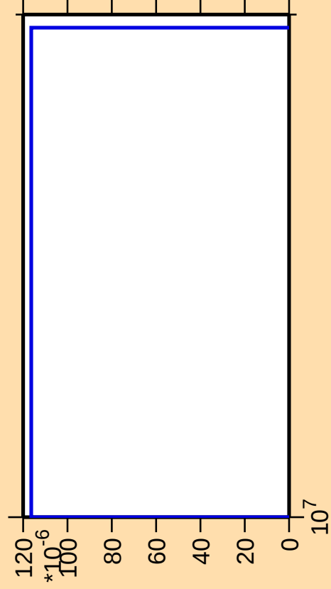
\Delta\sigma/\sigma vs. E for ^{96}\text{Y}(\text{mt } 11)
