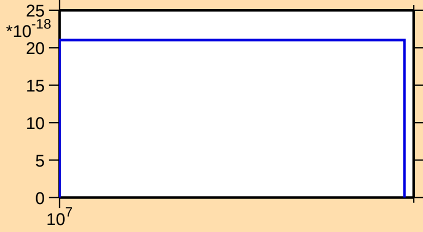
\sigma vs. E for ^{96}\text{Y}(\text{mt } 11)
