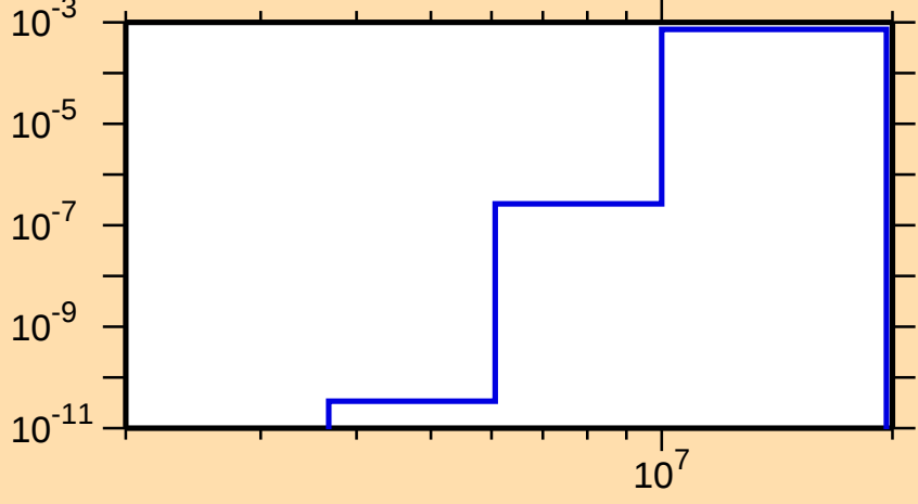
\sigma vs. E for ^{96}\text{Y}(n,\alpha)
