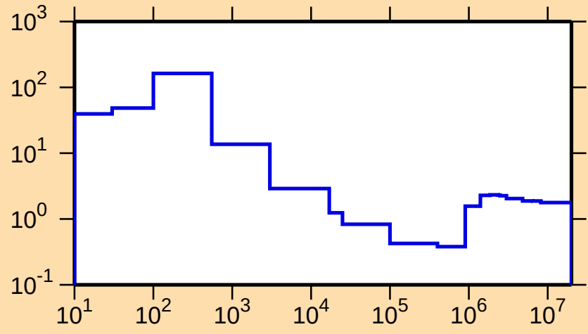
\sigma vs. E for ^{96}\text{Y}(n,\text{nonel.})
