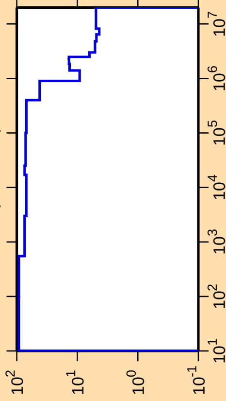
\Delta\sigma/\sigma vs. E for ^{96}\text{Y}(n,\text{nonel.})
